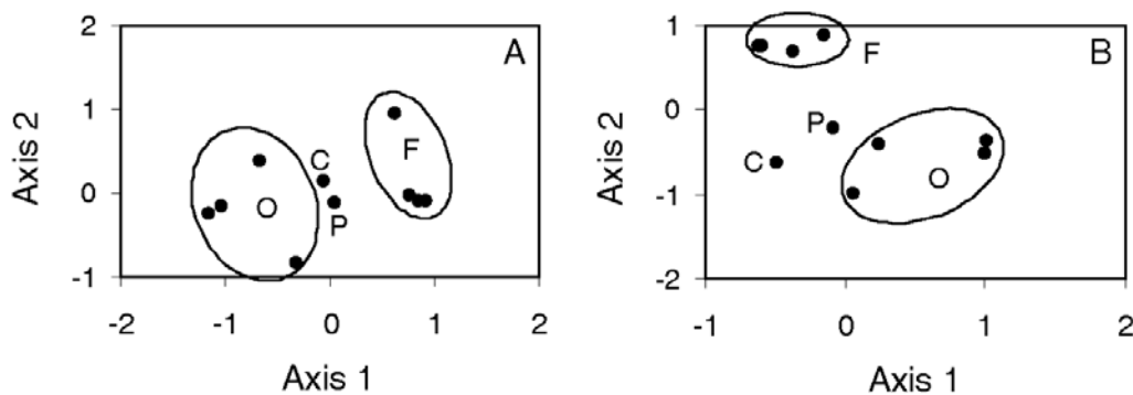
Figure 5. NMS ordination (Bray Curtis distance) using ranked abundances of destruent (A) and predator (B). O: open sites; F: forested sites; C: city centre; P: city periphery. Both ordinations favoured a three dimensional solution of which the first two axes are shown. The ellipses show the O and F sites.
