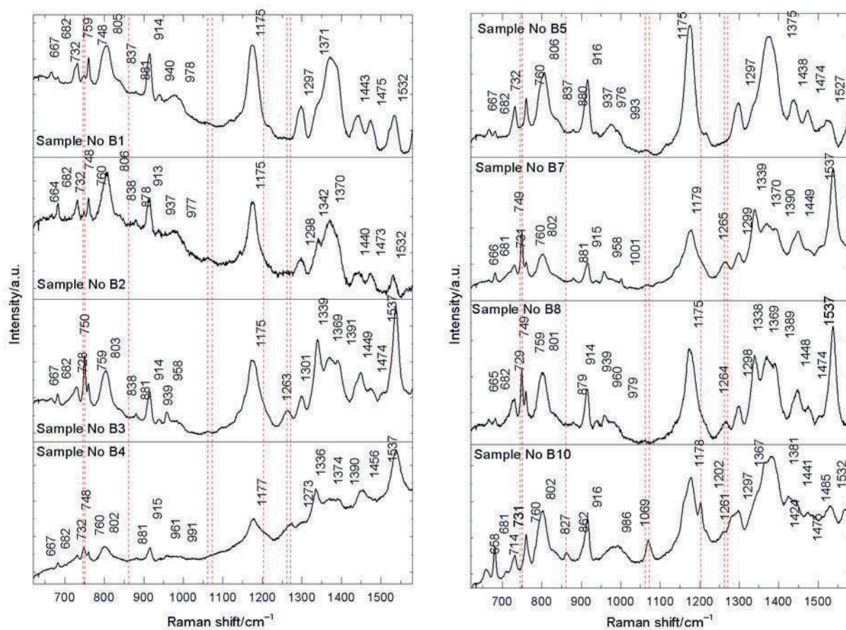
Fig. 3. SERS spectra of blue inks from group B (ballpoint pens) B1–B4 (left) and B5–B10 (right) in the range from 620 cm -1 to 1580 cm -1 . Dashed vertical lines represent the bands discussed in Table 2.
