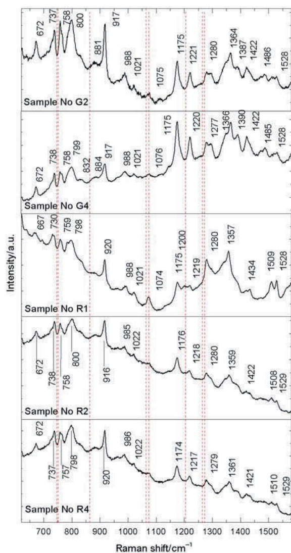
Fig. 4. SERS spectra of blue inks from group G (gel pens) and R (rollerball pens) in the range from 620 cm -1 to 1580 cm -1 . Dashed vertical lines represent the bands discussed in Table 2.
