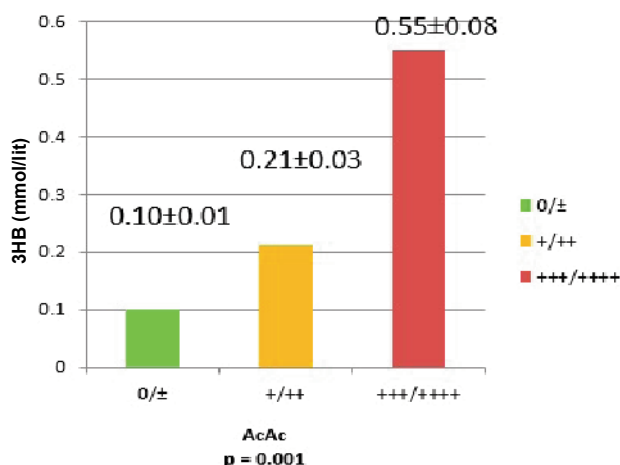
Figure 3. 3-β-hydroxybutyrate acid (3HB) levels depending on ketoneuria (AcAc, acetoacetate) severity.
