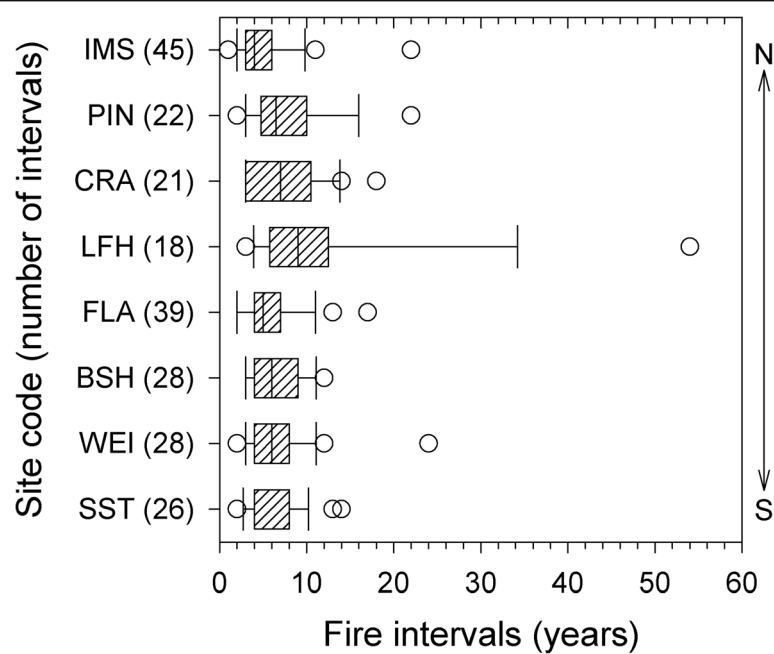
Fig. 7 Fire frequency at the forested eastern edge of the Palouse Prairie in Idaho, USA. The sites (Table 1) are arranged from north at the top to south at the bottom. Composite fire intervals were computed over 9 \pm 5 ha per site, during the analysis period from 1650 to 1900. Site codes on the vertical axis are followed by the number of fire intervals reconstructed during the analysis period. The boxes enclose the 25th to 75th percentiles and the whiskers enclose the 10th to 90th percentiles of the distribution of intervals. The vertical line across each box indicates the median fire interval, and all values falling outside the 10th to 90th percentiles are shown as circles
