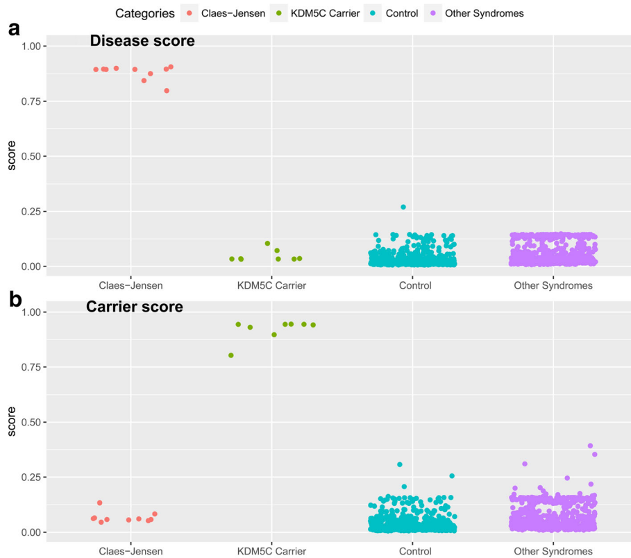
Fig. 4 Probability scores generated by the classification model: A multi-class SVM classifier concurrently generates two scores for every subject as the probability of having a DNA methylation profile similar to patients with Claes-Jensen syndrome ( a ) and healthy carriers of KDM5C mutations ( b ). y-axis represents scores 0–1, with higher scores indicating a higher chance of carrying a methylation profile related to any of the two statuses. The x-axis represents the classification scores for 10 patients with Claes-Jensen syndrome, 8 healthy carriers of KDM5C mutations, a total of 650 normal controls, and 587 patients with other conditions that present with intellectual disability as described in the “Methods” and “Results” sections. By default, the SVM classifier defines a cutoff of 0.5 for predicting the class; however, the vast majority of the tested individuals received a score close to 0 or 1. Therefore, for the purpose of better visualization, the points are jittered. Every point represents the probability score received for a single sample. This figure represents scores obtained by both the subjects in the training and testing cohorts
