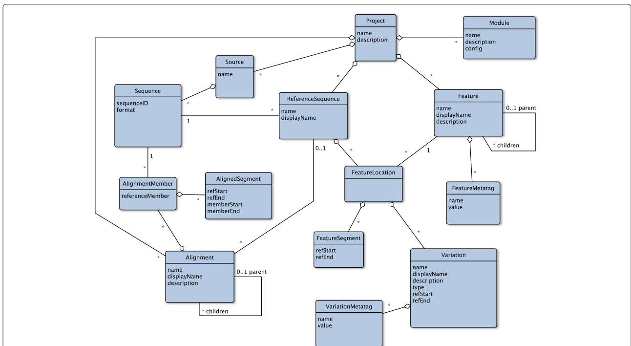
Fig. 1 The GLUE core schema. The main object types, fields and relationships in the core schema of GLUE, represented as a Unified Modelling Language (UML) entity-relationship diagram. Object types are represented as blue boxes with fields specified inside. Relationships between types are represented as lines connecting the associated object types. A diamond indicates a composition relationship. Relationship lines are annotated with “multiplicities” indicating how many objects participate in a single instance of the relationship; an asterisk indicates any number of objects
