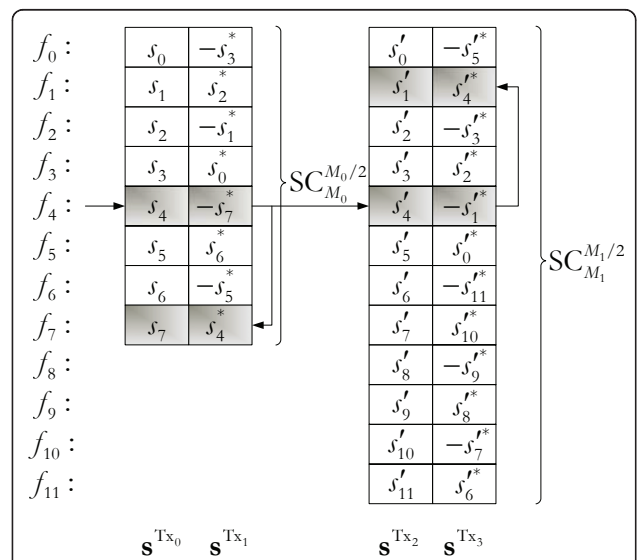
Figure 5 MU double SC-SFBC with incompatible pairing of subcarriers; example for M_0 = 8 , p_0 = 4 , M_1 = 12 , p_1 = 6 .
