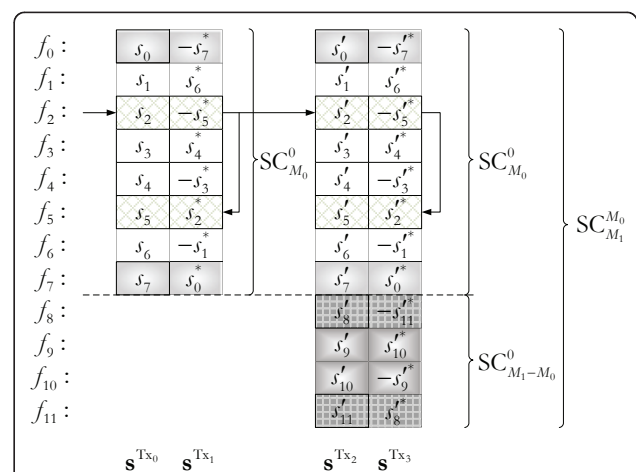
Figure 6 MU double SC-SFBC M_0 < M_1 , an example for M_0 = 8 , M_1 = 12 , p_0 = 0 , p_1 = 8 , n_0 = n_1 .
