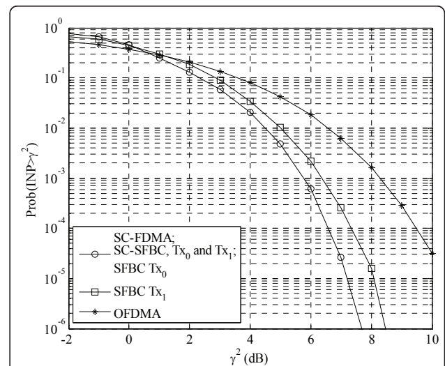
Figure 3 The distribution of the instantaneous normalized power (INP): SC-FDMA, SC-SFBC, classical SFBC, OFDMA.
