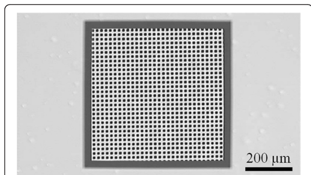
Figure 5 Locally opened through-silicon macropores. Optical microscope view of selective through-silicon macropore. This structure is achieved by alkaline etching (highly concentrated KOH solution at 80 °C) of the backside of the substrate through an oxide mask.
