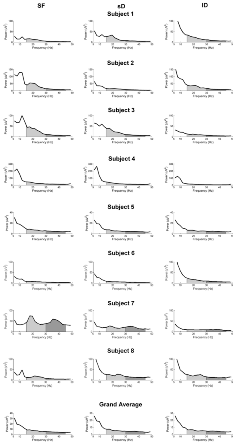
Figure 4 EEG spectral power plots. EEG spectral power during SF output (left panel), during sD force output (middle panel) and during ID force output (right panel) for single subjects and as grand average. The beta-range (15–30 Hz) is marked in light grey. The gamma-range (30–45 Hz) is marked in dark grey.
