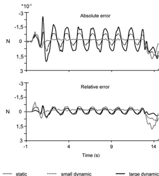
Figure 1 Performance Analysis. Motor performance error, upper panel absolute error, lower panel relative error (the error after normalization to the amplitude of the force) for 8 subjects (Grand average). The static force ( SF ) condition is marked as grey line, the small dynamic ( sD ) condition as dotted black line and large dynamic ( ID ) condition as thick black line.
