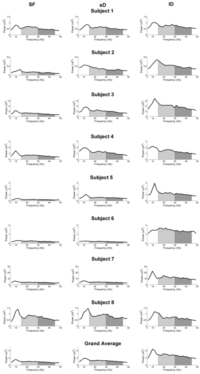
Figure 5 EMG spectral power plots. EMG spectral power during SF output (left panel), during sD force output (middle panel) and during ID force output (right panel) for single subjects and as grand average. The beta-range (15–30 Hz) is marked in light grey. The gamma-range (30–45 Hz) is marked in dark grey. Note the highest EMG SP during ID condition.
