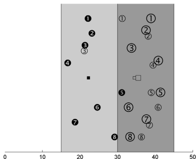
Figure 3 Center of gravity for frequency. (a) Individual frequency values of maximum coherence (centre of gravity) calculated for the whole range study (15–45 Hz). Each subject is represented by a number. Filled circles and square: individual values and their mean for the SF condition. Small empty circles and square: values and mean for the sD condition. Large empty circles and square: values and mean for the ID condition. The beta-range (15–45 Hz) is marked in light grey, the gamma-range (30–45 Hz) in dark grey. Note that the frequency values for the both dynamic conditions are systematically higher than for the static condition, but there are no differences of the frequency values between both dynamic conditions.
