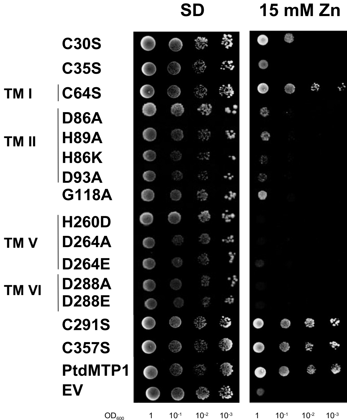
Figure 2 Effect of amino acid substitution on the ability of PtdMTP1 to protect against Zn 2+ toxicity in yeast. The Zn-hypersensitive yeast strain zrc1Δ , transformed with pYES2 bearing the mutated variants of PtdMTP1 was grown at 30°C in SD with 2% galactose (SD) until O.D. 600 nm = 1. Serial dilutions were spotted on SD or on SD + 15 mM ZnCl 2 (15 mM Zn). Photographs were taken after 6 days of growth at 30°C. For each mutation different yeast transformants were used and gave the same results. The amino acid substitutions along with their topological positions are shown on the left. EV: empty vector; PtdMTP1: wild type protein.
