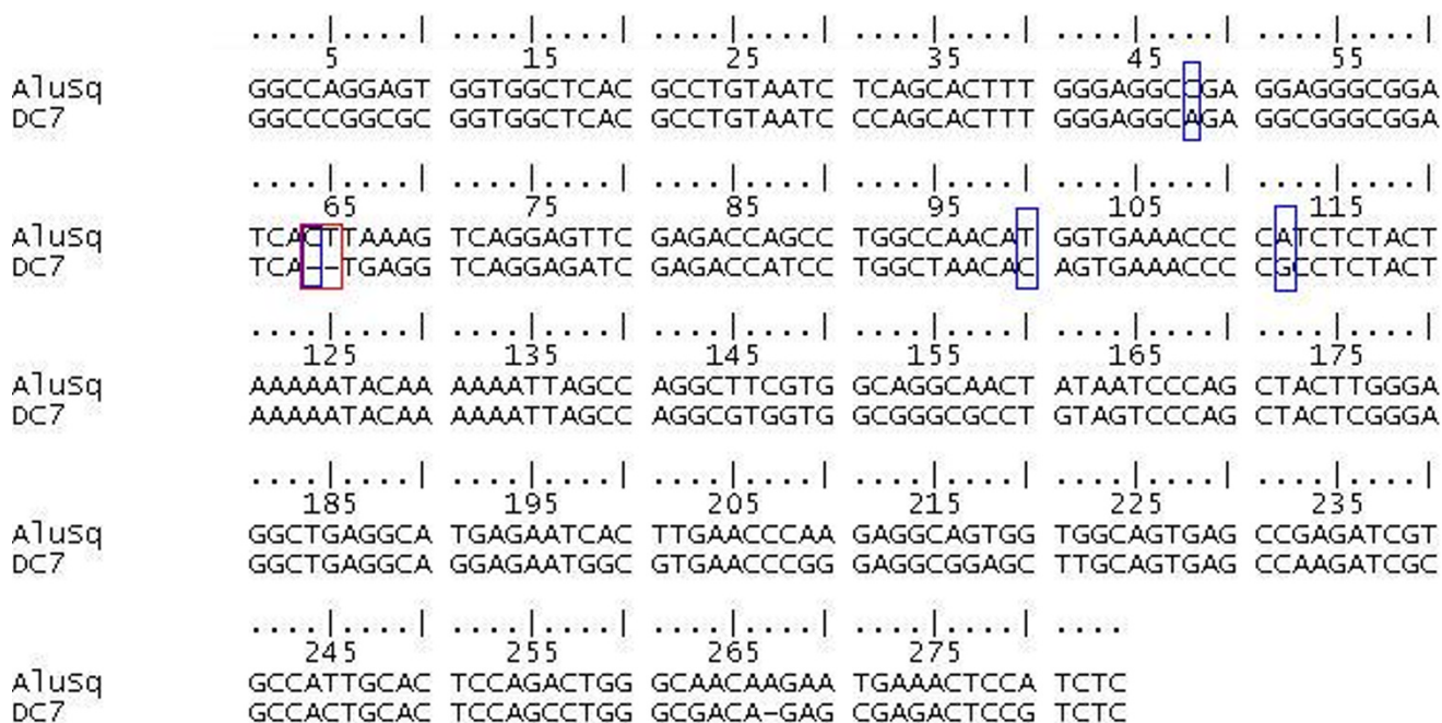
Figure 3 Alignment of the chimpanzee AluYh3a1 element DC7 and the AluSq element present at the orthologous position in the human genome. Diagnostic positions for AluYh3a1 are shown in blue boxes, the characteristic deletion of AluSq is shown in a red box. This case represents an example of complete gene conversion replacing an Alu element from an old subfamily with one from a younger subfamily.
