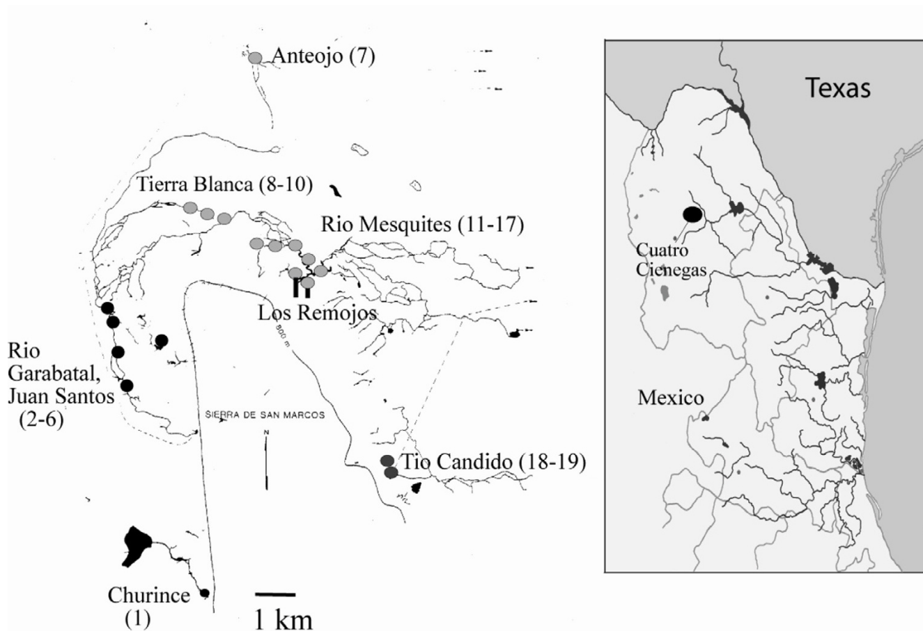
Figure 1 Collecting sites of Mexipyrghus churinceanus from spring-fed habitats in the Cuatro Ciénegas valley located in the center of the Chihuahuan desert of northeastern Mexico. These pools and streams are arrayed around the Sierra de San Marcos that bisects the center of the valley. Population numbers are shown on the map and referred to in Table 1.
