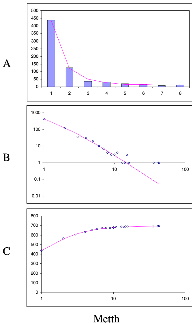
Figure 12 Fit of empirical domain family size distributions to the second-order balanced linear BDIM: the thermophilic euryarchaeon Methanothermobacter thermautotrophicus . The panels and the designations are as in Fig. 6. B. Magenta line: f_i = 2753\Gamma(i+0.12)/\Gamma(i+3.00)
