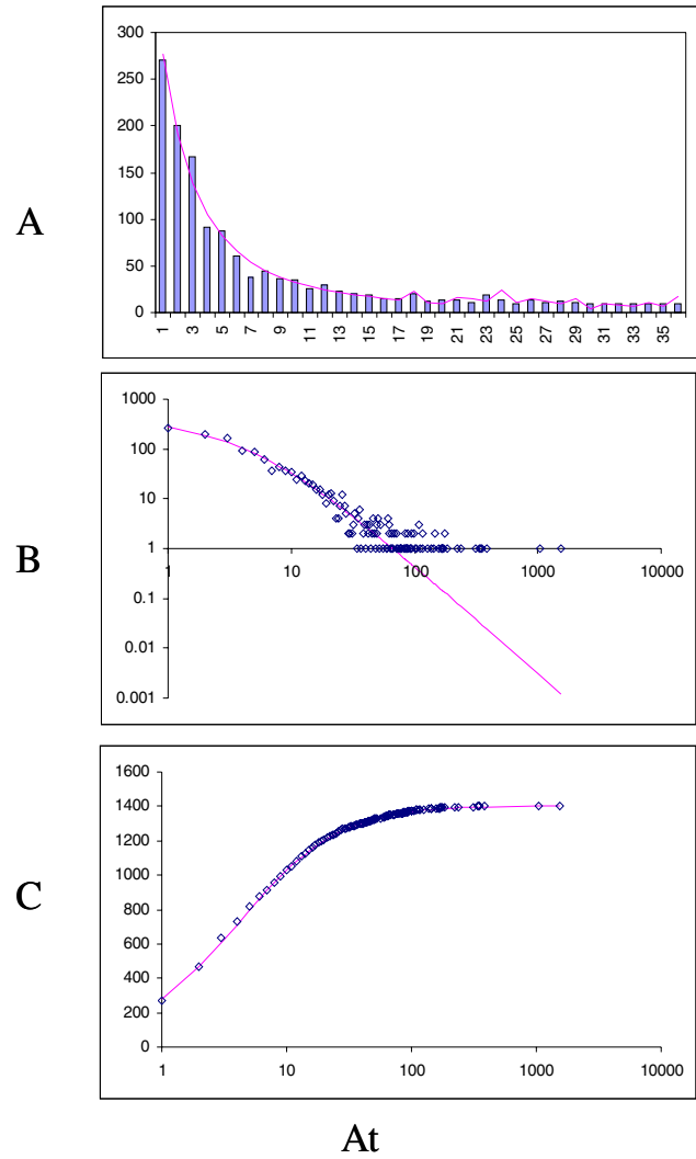
Figure 9 Fit of empirical domain family size distributions to the second-order balanced linear BDIM: the thale cress Arabidopsis thaliana . The panels and the designations are as in Fig. 6. B. Magenta line: f_i = 10750\Gamma(i+3.80)/\Gamma(i+5.98)
