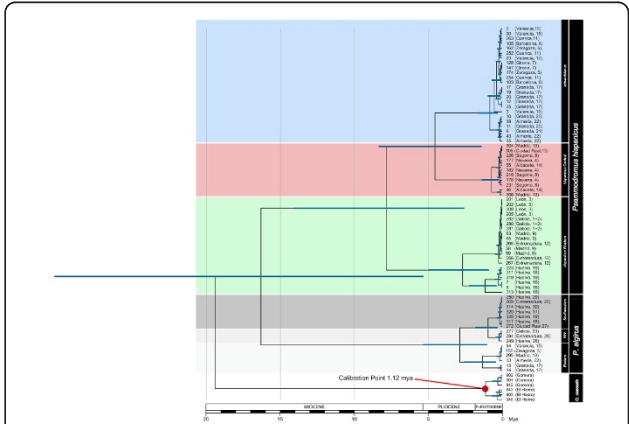
Figure 3 Bayesian relaxed-clock timetree of the genus Psammodromus based on the combined data set. The sister group to Psammodromus ( Gallotia ) was used as an outgroup and as calibration point for the molecular clock. The species, subspecies, and lineage name and the specimen's reference number are given. The sample location and the population number are indicated in brackets. Estimated ages and 95% confidence intervals are indicated.
