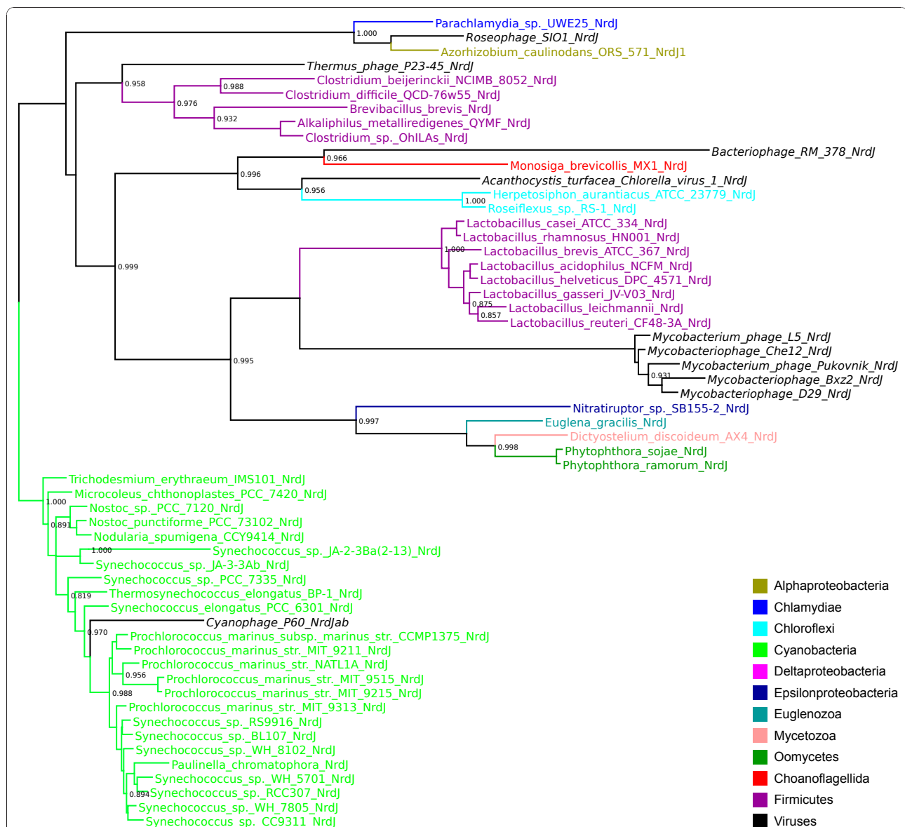
Figure 7 Phylogeny of monomeric class II RNR from eukaryotes together with their most similar bacterial sequences. A PhyML ULS phylogeny from an alignment of protein sequences of monomeric class II RNR enzyme from eukaryotic genomes and genomes containing similar sequences. The arrows indicate eukaryotic sequences. Top level groups from the NCBI taxonomy have been colour-coded; viruses are in italics. The tree is not formally rooted; the pseudoroot is placed so as to be consistent with the global phylogeny in Figure 1c.
