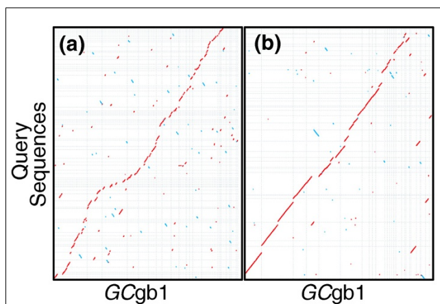
Figure 3 Comparison of Forge Sanger/454/Illumina assemblies against GCgb1 . Alignments of scaffolds greater than 100 kb - (a) 'Sanger/454/IlluminaDA' (approximately 24 Mb on 80 scaffolds) and (b) 'Sanger/454/IlluminaPA' (approximately 28.7 Mb on 46 scaffolds) - on the y-axis against the manually finished genome sequence ( GCgb1 ) on the x-axis.
