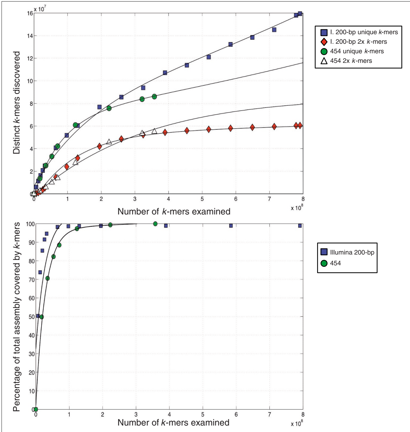
Figure 4 Assessing the discovery of unique read information between the Illumina and 454 platforms. (a) Raw reads were processed into overlapping 28-bp k-mers, and any k-mer that varied from all other k-mers by at least 1 bp was accepted as new sequence information. The analysis was done separately for unique k-mers and those that occurred at least twice (2x k-mers). (b) MAQ was then used to map these k-mers to the reference genome sequence and the rate at which new coverage was generated was plotted against the number of k-mers examined.
