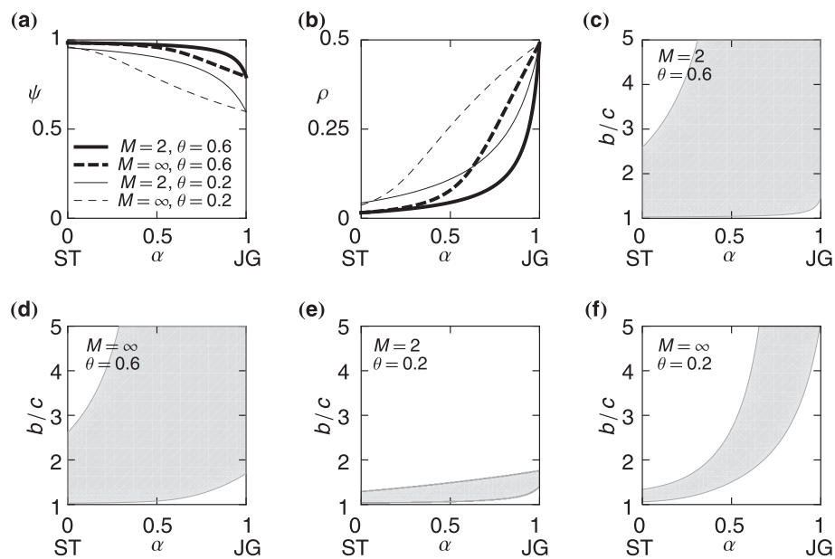
Figure 6 Equilibria and the stability conditions for a population of DISC players under MX. (a) Cooperativeness ( \psi ) and (b) ingroup bias ( \rho ). In (a) and (b) , we set (M, \theta) = (2, 0.6), (\infty, 0.6), (2, 0.2), and (\infty, 0.2) . (c)–(f) Stability conditions. The homogeneous population of DISC players is stable in the shaded parameter regions. We set (c) (M, \theta) = (2, 0.6) , (d) (M, \theta) = (\infty, 0.6) , (e) (M, \theta) = (2, 0.2) , and (f) (M, \theta) = (\infty, 0.2) .
