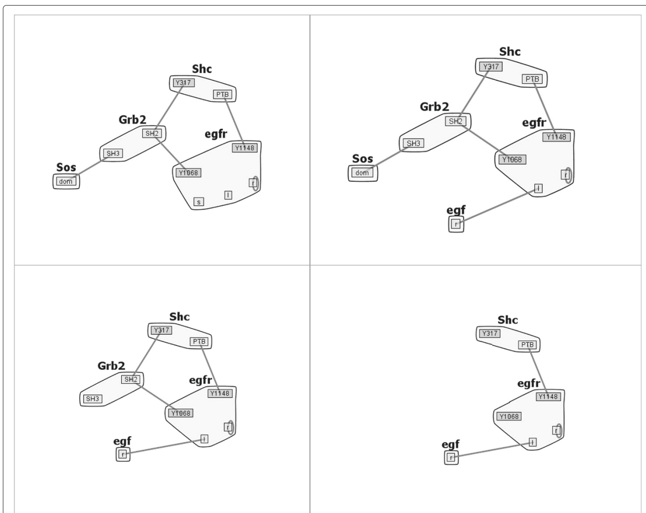
Figure 3 EGFR Models. Four sample multiples from the EGFR family of models sorted by similarity score relative to the most complete model (upper left). The most complete model generates a reaction network with 356 species and 3,749 reactions.
