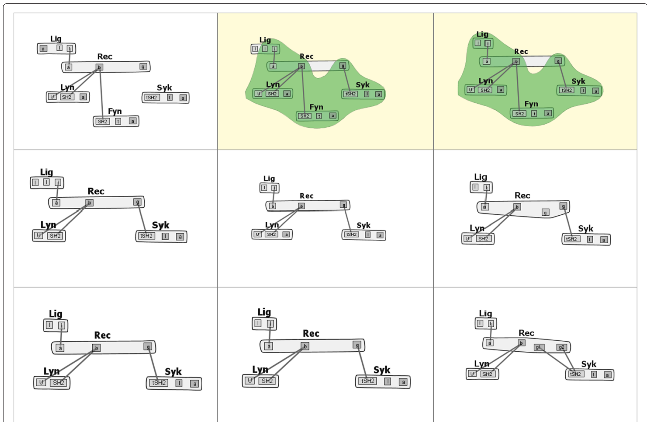
Figure 6 fceri Similarity Comparison. A similarities comparison within the fceri model family, highlighting the similarities between the fceri_fyn and fceri_fyn_trimer models. The fceri_fyn model (top right) generates a reaction network with 1,281 species and 15,256 reactions, while the fceri_fyn_trimer model (top middle) generates a reaction network with 20,881 species and 407,308 reactions.
