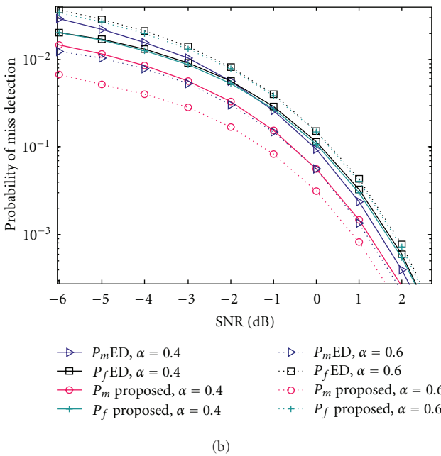
FIGURE 4: The missed detection and false alarm probabilities under different preferences.
