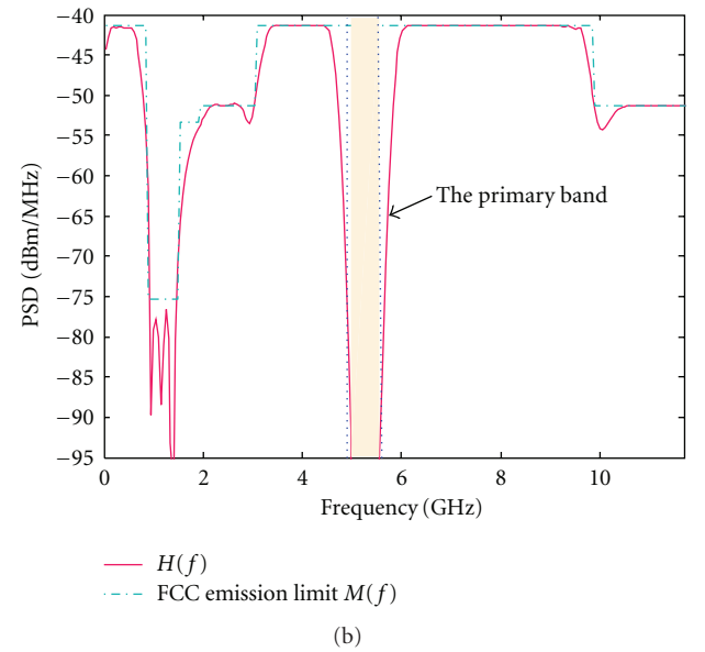
FIGURE 6: The designed UWB signals under different applications. (a) UWB waveform without regulatory emission limits. (b) UWB waveforms under FCC emission template. Notice that the total number of the basis functions is 64 in (b).
