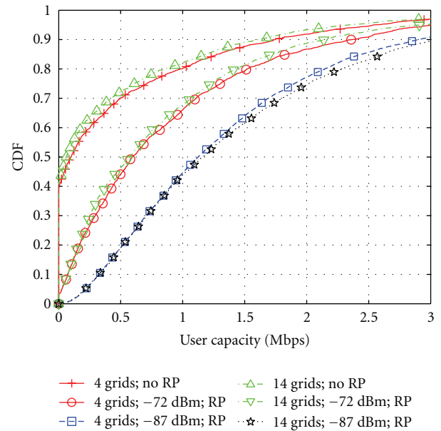
FIGURE 8: CDFs showing downlink user capacity only for affected macro UEs for a system with resource partitioning compared against a system without resource partitioning.
