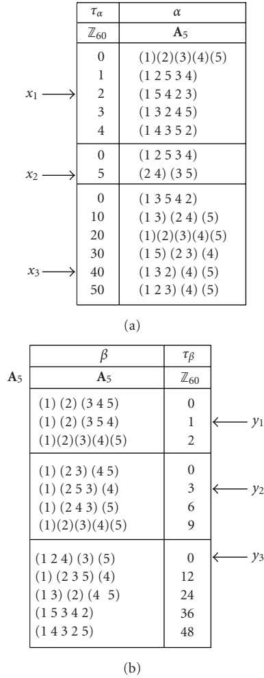
FIGURE 13: Two logarithmic signatures of A_5 .
