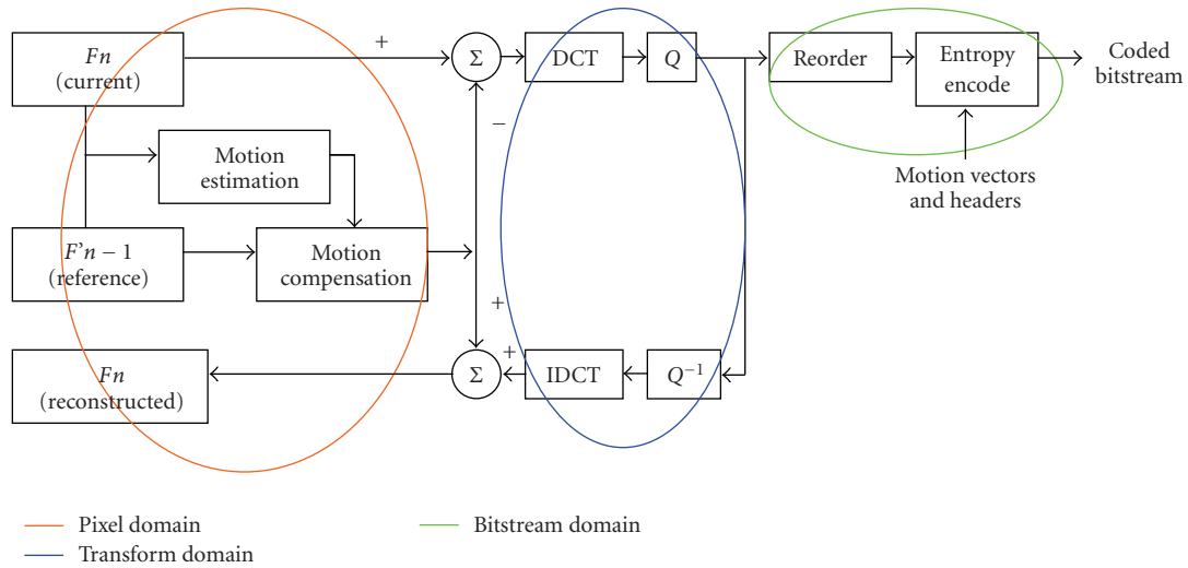
FIGURE 1: Video encoder highlighting opportunities for encryption.
