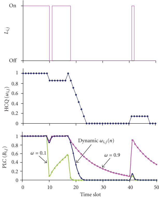
FIGURE 7: Evolution of multi-scale locality in terms of PLC and HCQ.
