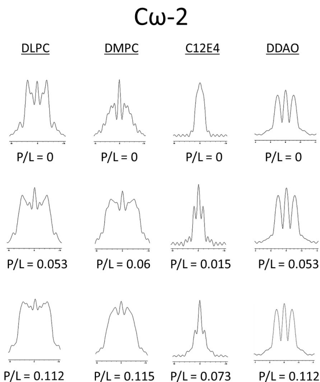
Fig. 2. Dipolar coupling slices of the C_{\omega-2} at 30 °C.
