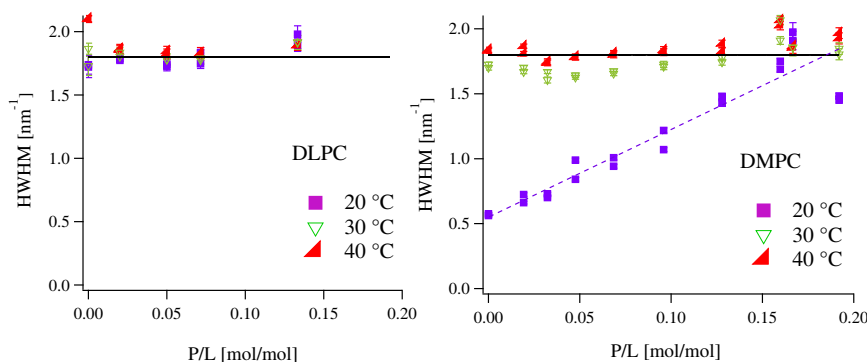
Fig. 4. Width of the chain peak for DLPC (left) and DMPC (right) bilayers as a function of the GramA doping at three temperatures.
