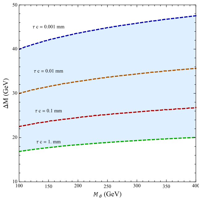
Fig. 11 Region of parameter space in the light-stop window of the MSSM ( left ) corresponding to scalar top decay lengths between 0.001 and 1 \text{ mm} . On the right we show a scenario where the width of the
