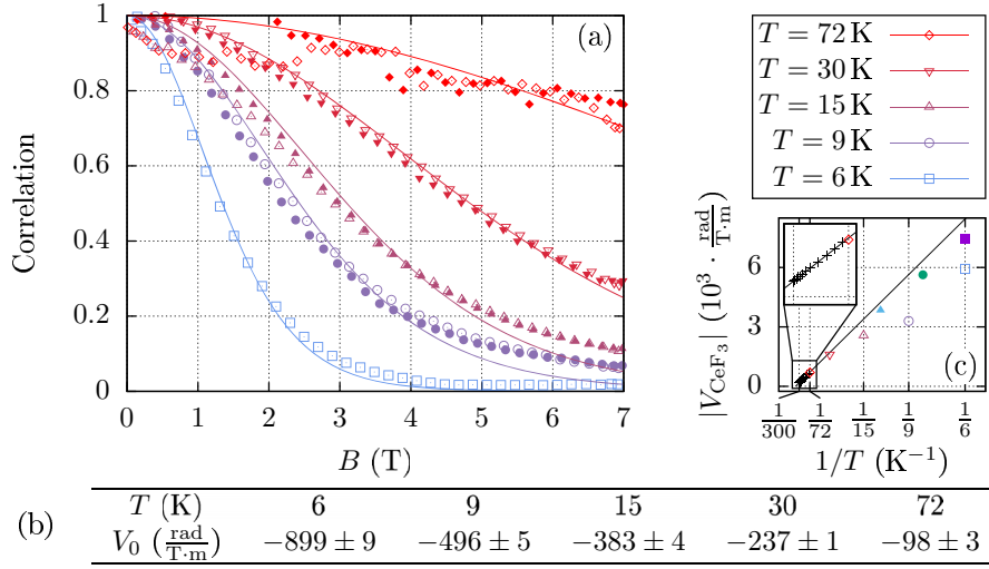
Fig. 5. (a) Correlations of the transmission speckle for a sample consisting of 3.8 vol% TiO 2 and 5.3 vol% CeF 3 solved in 90.9 vol% glycerol as a function of the magnetic field for different temperatures. Open symbols: increasing field, correlation with the first image; filled symbols: decreasing field, correlation with the last image. (For T = 6 K, only the measurement with increasing field was evaluated since problems with the cryostat occurred during the decrease of the field.) The decorrelations are fitted (solid lines) as in Figure 4. (b) Measured Verdet constant V_0 for the different temperatures. (c) Recalculated bulk Verdet constant of CeF 3 V_{\text{CeF}_3} (using the measured E_V at 72 K for all temperatures) as a function of the inverse temperature (open symbols). For comparison the high temperature dependency of the Verdet constant (between 77 K and 300 K) measured in reference [16] (black crosses) is plotted and fitted by V \propto 1/T (solid black line) and the low temperature data measured in Figure 6 are shown (filled symbols).
