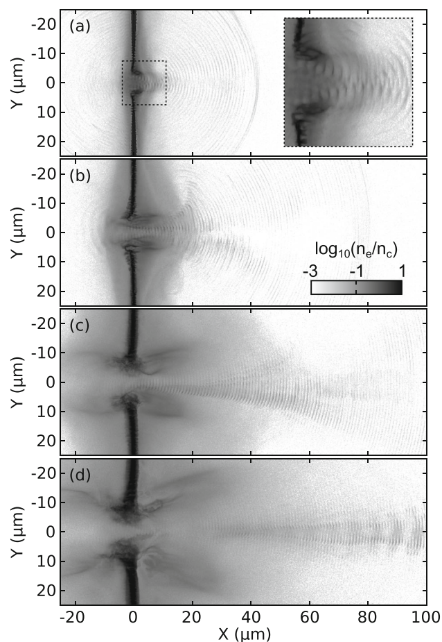
Fig. 9 2D simulation results showing electron density for a pulse with peak a_0 = 20 interacting with an initially solid density aluminium target at t = \tau_L/4 for: a \tau_L = 100 fs; b \tau_L = 200 fs; c \tau_L = 400 fs; and, d \tau_L = 600 fs. The inset in a shows a zoomed-in region of the electron density in the region of the focal spot, corresponding to the black dashed box. The thickness of the target is adjusted such that the target undergoes RSIT at t = 0 . See Supplementary Material for the simulation parameters
