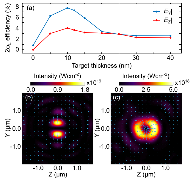
Fig. 11 Example 3D simulation results [32]. a Laser energy conversion efficiency into 2\omega_L light, shown for the two orthogonal polarization components in absolute electric field terms. b–c Time-integrated spatial profile, in the Y – Z plane, of the intensity of 2\omega_L light for: b a 5 nm-thick target; and c a 20 nm-thick target, detected at X = 10 \mu\text{m}
