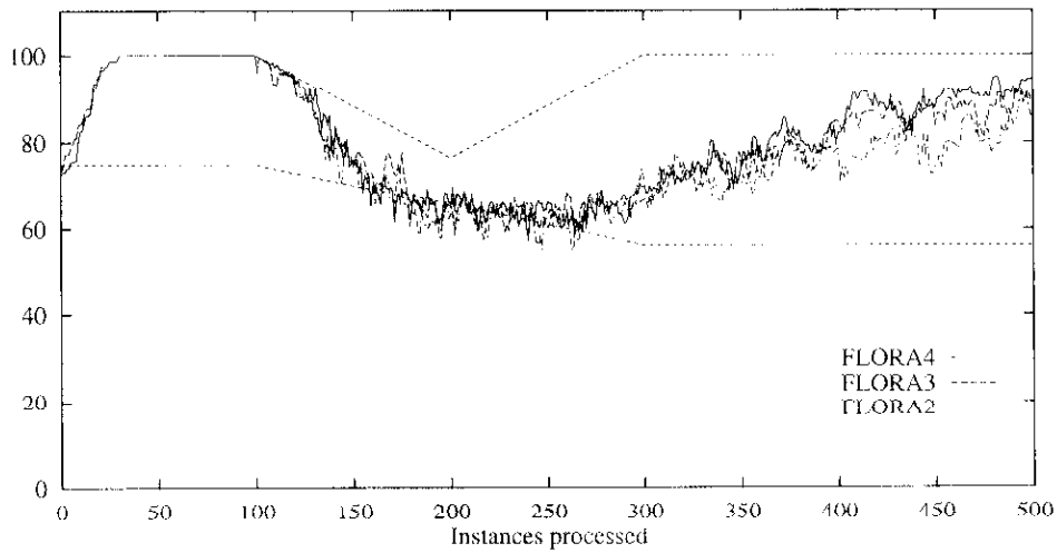
Figure 15. Performance for \Delta x = 200 .
