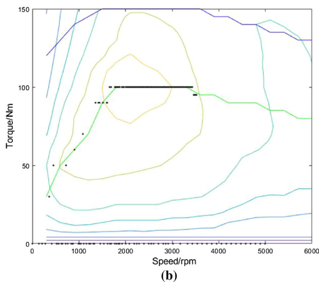
Fig. 6 Working point distribution of P2 HEV. a Working points of DDA method. b Working points of rule-based strategy
