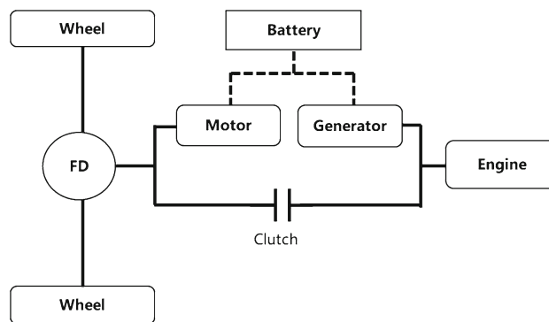
Fig. 4 Architecture of SP HEV
