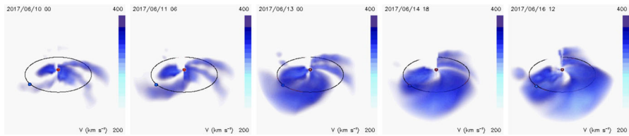
Fig. 72 A sequence of tomographic reconstructions of the solar wind speed using IPS observations, from a viewpoint at 3 AU, 30^\circ above the ecliptic and 45^\circ ahead of the Earth, for June 10–16, 2017, from the UCSD CASS IPS website ( http://ips.ucsd.edu/ )
