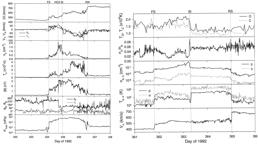
Fig. 38 Left: An interaction region observed in November 1992 at 5 AU, 23^\circ\text{S} . The parameters shown are: The solar wind speed and transverse and normal components, density, temperature, magnetic field intensity and polar and azimuthal angles, and the total pressure. Vertical lines indicate crossings of the forward shock (FS), heliospheric current sheet (HCS), stream interface (SI), and reverse wave (RW). Right: An interaction region observed in December 1992 showing the solar wind oxygen and carbon freezing in temperatures, alpha to proton ratio, densities and temperatures, and the alpha particle speed. Note the changes in the O and C freezing-in temperatures (i.e., charge states), and alpha/proton ratio at the stream interface indicating the different origins at the Sun of plasma on either side of the interface. Images reproduced with permission from [left] Forsyth and Gosling (2001), copyright by Springer; and [right] Wimmer-Schweingruber et al. (1997), copyright by AGU
