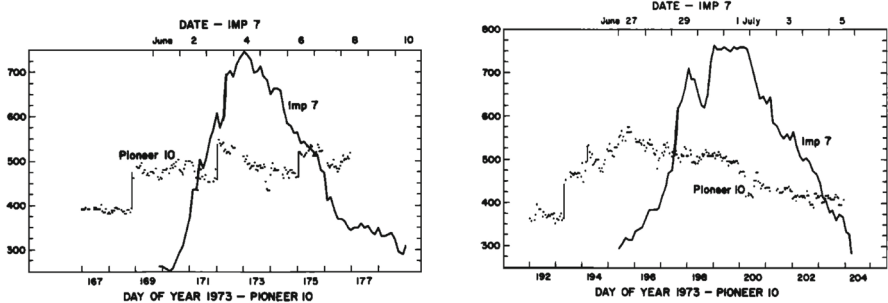
Fig. 27 Two high-speed streams observed at IMP 7 and Pioneer 10 at 4 AU, showing the steepening of the stream leading edge, including the formation of abrupt speed jumps associated with shocks, and the reduction in the peak speed of the stream. Image reproduced with permission from Gosling et al. (1976), copyright by AGU
