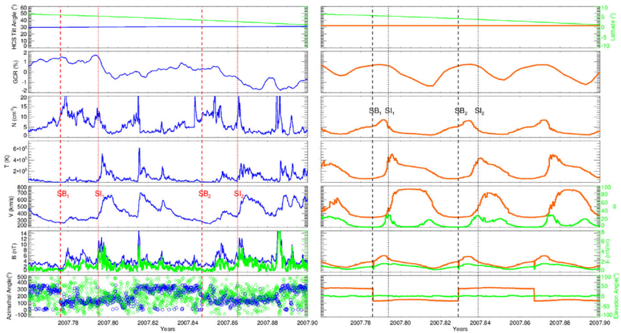
Fig. 60 Solar wind and GCR observations (left) near Earth during a period in 2007, and corresponding modeled parameters. Note that the GCR modulations are unrelated to enhancements in the magnetic field intensity and sector boundary crossings, and commence in the vicinity of stream interfaces/fast stream leading edges, consistent with the observations in the left panel and discussed in the text. See Guo and Florinski (2016) for a detailed description of the parameters shown in the figure. Image reproduced with permission from Guo and Florinski (2016), copyright by AAS
