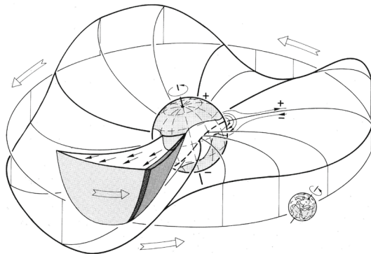
Fig. 10 Configuration in the inner heliosphere of a "ballerina skirt" heliospheric current sheet (Alfvén 1977) extending above the streamer belt near solar minimum (for A > 0 solar magnetic field polarity, i.e., outward field at the north pole), which lies ahead of a high-speed stream (drawn truncated at high latitudes) from an equatorward extension of a northern polar coronal hole. The dark shaded region is the interaction region. Image reproduced with permission from Schwenn (1990), copyright by Springer
