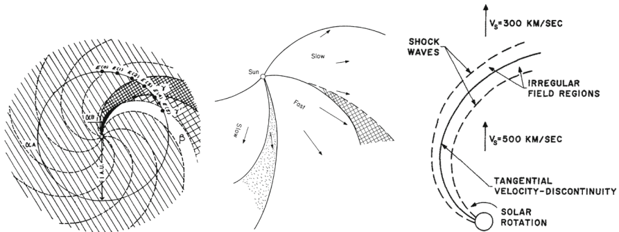
Fig. 12 Three sketches of the interaction between slow and fast solar wind streams. Left: Formation of a turbulent compression region \gamma and cavity \beta at leading and trailing edges of a high-speed stream, respectively. Image reproduced with permission from Sarabhai (1963), copyright by AGU. Center: A region of compressed plasma (hatched) at the leading edge of the fast stream and a rarefaction (dotted) at the trailing edge. Image reproduced with permission from Parker (1965a), copyright by D. Reidel. Right: A region of turbulence caused by the Kelvin–Helmholtz instability at the stream interaction, also suggesting the formation of shocks at the boundaries of the interaction region and a tangential discontinuity separating slow and fast solar wind. Image reproduced with permission from Dessler and Fejer (1963), copyright by Elsevier
