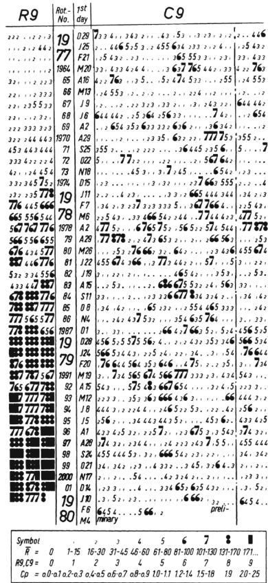
Fig. 5 Left: Distribution of geomagnetic disturbances in 1882–1903 according to the heliographic longitude of the center of the Sun’s disk at time of their commencement. Image reproduced with permission from Maunder (1904), copyright by RAS. Right: 27-day (Bartels rotation) stackplot of the daily C9 geomagnetic index and 3-day mean sunspot number (R9) for 1977–early 1980. Note that intervals of recurrent activity tend to be most prominent at times of lower solar activity levels, while isolated sporadic storms are more prominent at higher activity levels. A current figure in a similar format is available at http://www-app3.gfz-potsdam.de/kp_index/r9c9.pdf
