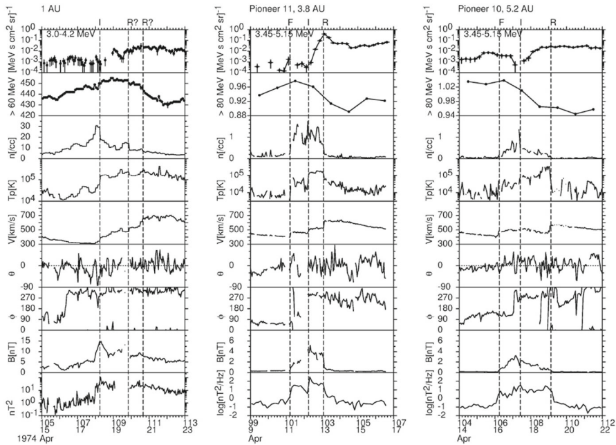
Fig. 57 Observations of energetic particles, solar wind plasma and magnetic field (in HSE co-ordinates) associated with passage of the same interaction region at 1 AU, Pioneer 11 at 3.8 AU, and Pioneer 10 at 5.2 AU. Forward (F) and reverse (R) shocks and stream interface crossings (I) are indicated. The bottom panels indicate magnetic field turbulence levels. The GCR modulation associated with the interaction region is shown in the second graph in each panel
