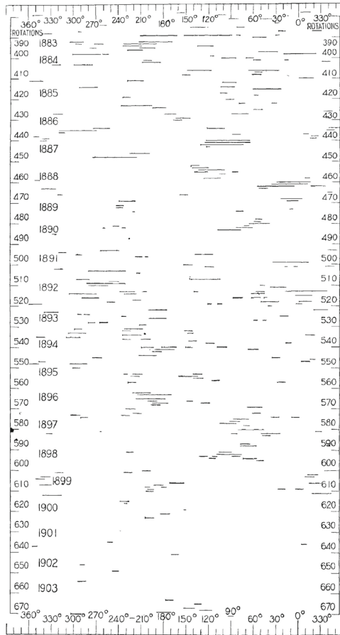
Fig. 5 Left: Distribution of geomagnetic disturbances in 1882–1903 according to the heliographic longitude of the center of the Sun’s disk at time of their commencement. Image reproduced with permission from Maunder (1904), copyright by RAS. Right: 27-day (Bartels rotation) stackplot of the daily C9 geomagnetic index and 3-day mean sunspot number (R9) for 1977–early 1980. Note that intervals of recurrent activity tend to be most prominent at times of lower solar activity levels, while isolated sporadic storms are more prominent at higher activity levels. A current figure in a similar format is available at http://www-app3.gfz-potsdam.de/kp_index/r9c9.pdf
