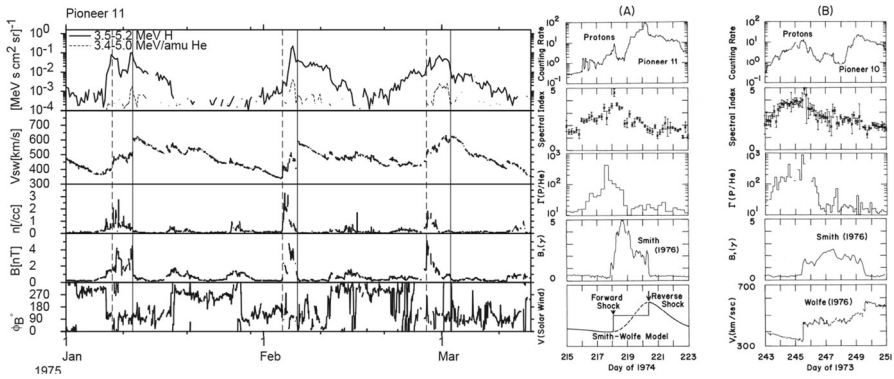
Fig. 45 Left: Stream interaction region-associated particle enhancements (3.5–5.2 MeV protons and 3.4–5.0 MeV/n He) observed by the Goddard experiment on Pioneer 11 at \sim 4.6 AU in early 1975, showing intensity increases in the vicinity of forward and reverse shocks (dashed and solid vertical lines, respectively). Right: 0.5–1.8 MeV proton intensity in the vicinity of the forward and reverse shocks of two interaction regions observed by Pioneer 10 or 11. Other parameters shown are the proton differential spectrum power law index, proton/alpha particle ratio ( \Gamma ), magnetic field intensity and solar wind speed. Note that the reverse shock particle enhancement has a harder spectrum (smaller spectral index) and smaller proton/alpha particle ratio than the enhancement at the forward shock. Images reproduced with permission from [left] Richardson (2004), copyright by Kluwer; and from [right] Barnes and Simpson (1976), copyright by AAS
