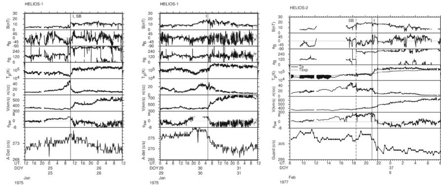
Fig. 55 Examples of GCR depression onsets associated with interaction regions observed by the Helios spacecraft. ‘I’ indicates the stream interface and ‘SB’ a sector boundary crossing. The GCR intensity is given by 15 min averages of the anti-coincidence guard of the University of Kiel instruments. Note that the depressions tend to commence in the vicinity of the stream interface/leading edge of the high-speed stream, and are not clearly associated with enhanced fields in the interaction region or sector boundaries (absent in the center panel). Image reproduced with permission from Richardson (2004), copyright by Kluwer
