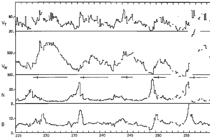
Fig. 13 A 35-day interval of Mariner 5 data, showing several high-speed streams separated by periods of slower solar wind. The solar wind thermal speed ( V_T ), solar wind speed ( V_W ), density ( N ) and magnetic field intensity ( B ) are shown. Note that the density peaks tend to occur at or just ahead of the start of the speed gradients, and the magnetic field peaks occur later, within the gradient. The horizontal lines indicate where Alfvén waves were identified, with thicker lines indicating where the strongest waves were observed, in the speed gradients. Image reproduced with permission from Belcher and Davis (1971), copyright by AGU
