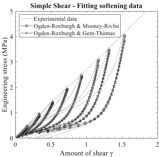
Fig. 19 Fitting the Ogden–Roxburgh model to the softening data
