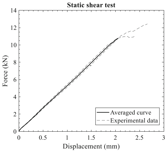
Fig. 8 Static shear test results
