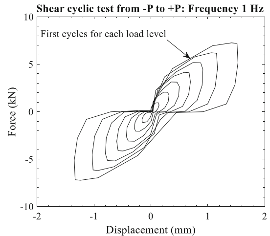
Fig. 11 Cyclic shear test results from -P to +P at 1 Hz
