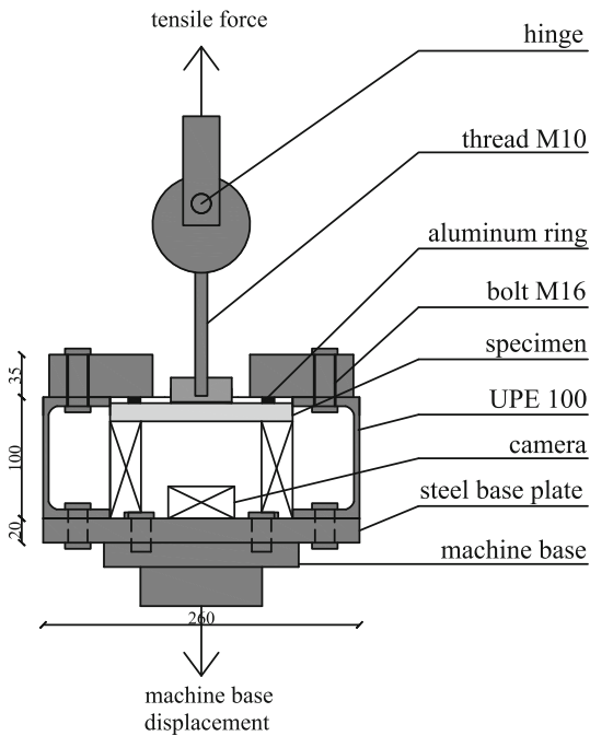
Fig. 7 Simplified sketch of the tensile test set-up
