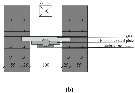
Fig. 3 Simplified sketch of the shear load application: a isometric view and support conditions, b top view
