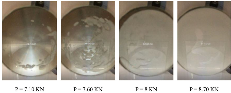
Fig. 14 The whitening phenomenon under tensile static loading
