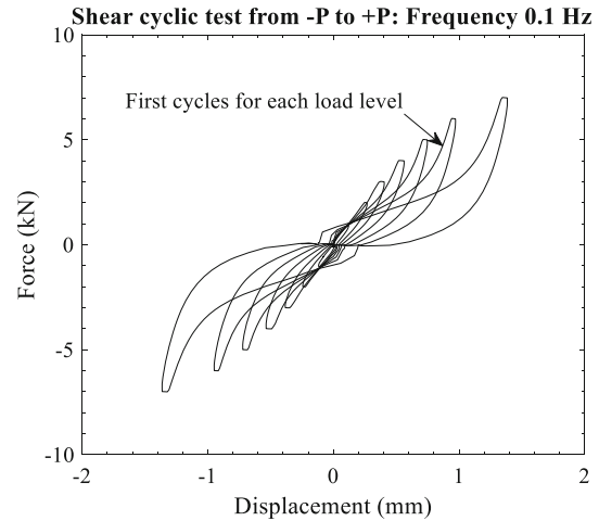
Fig. 10 Cyclic shear test results from -P to +P at 0.1 Hz
