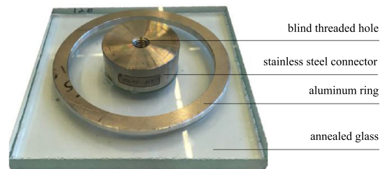
Fig. 6 Glass specimens subjected to tensile tests
