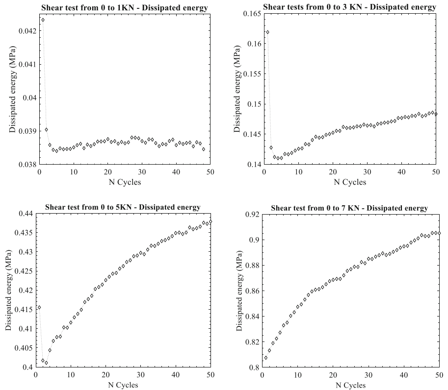
Fig. 18 Energy dissipation analysis
