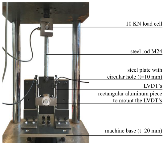
Fig. 2 Shear test set-up
