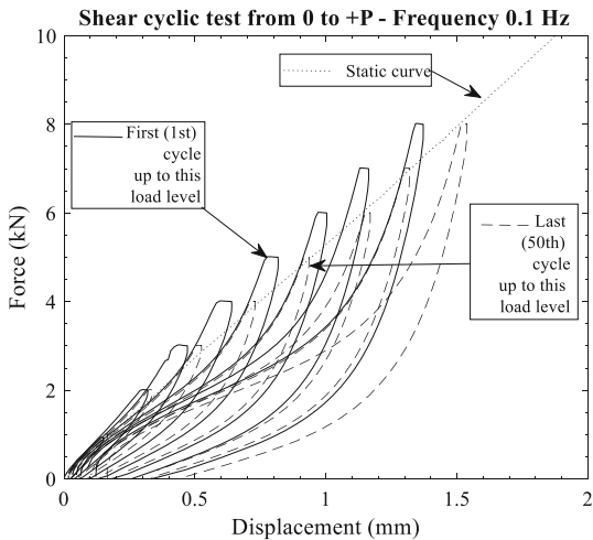
Fig. 9 Cyclic shear test results from 0 to +P at 0.1 Hz
