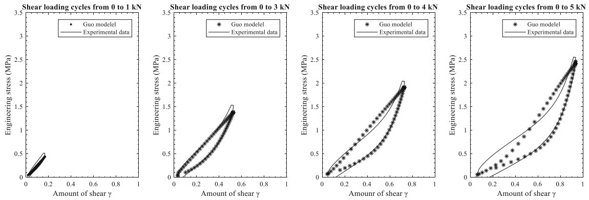
Fig. 20 Fitting the Guo model to the experimental softening data
