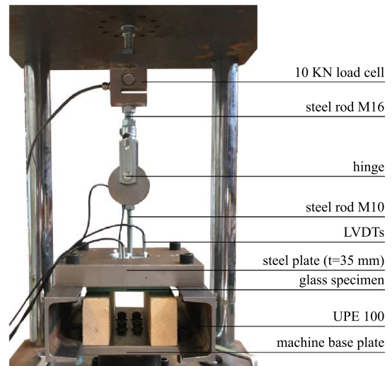
Fig. 5 Tensile test set-up
