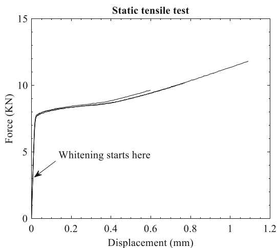
Fig. 13 Static tension test results
