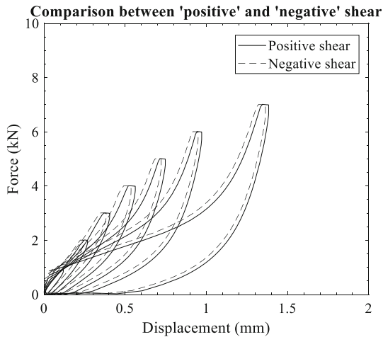
Fig. 12 Comparison between 'positive' and 'negative' shear
