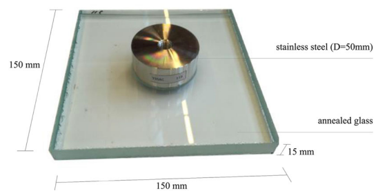
Fig. 1 Glass specimens with laminated circular connectors
