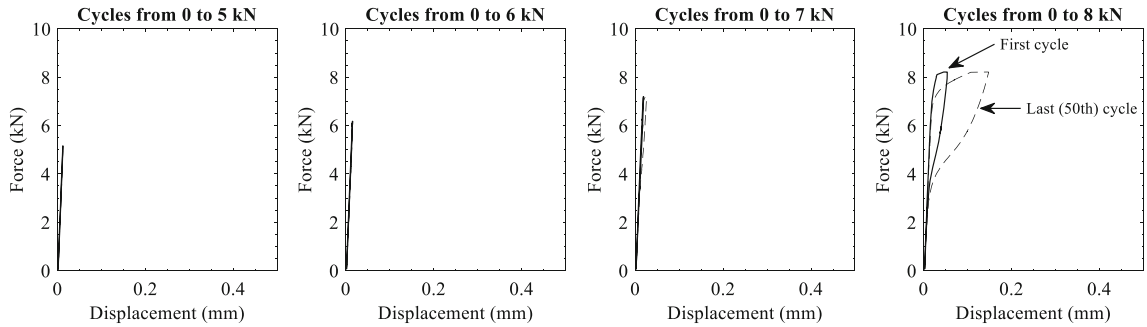
Fig. 15 Tensile cyclic loading test results
