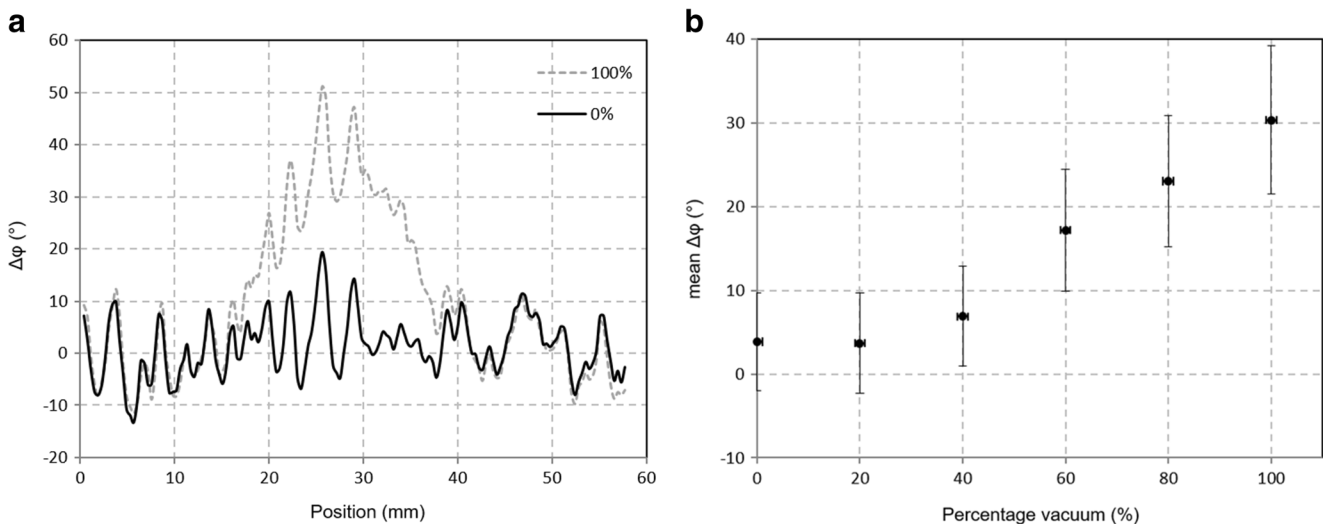
Fig. 7 (a) phase contrast profiles taken across the defect region under vacuum loading conditions of 100% vacuum and 0% vacuum and (b) the mean phase contrast between defect and non-defect regions taken across the width of the defect related to partial vacuum percentage applied
