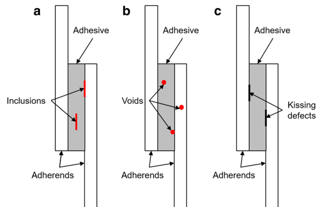
Fig. 2 Three categories of defects typically found in adhesive joints; (a) inclusions, (b) voids and (c) kissing defects
