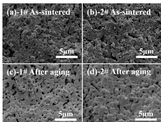
Fig. 3 Fracture surfaces of the ceramics (1# and 2#) before and after thermal aging at 1300 °C for 24 h.
