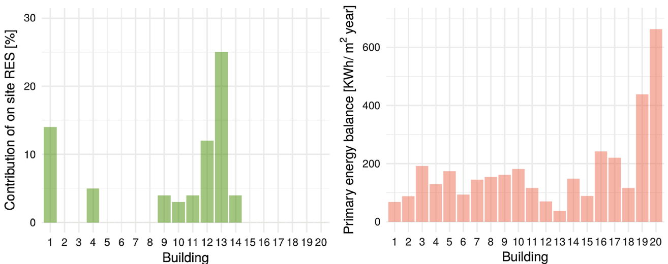
Fig. 17 Percentage of primary renewable energy generated on-site (left plot) and the overall primary energy balance (right plot)
