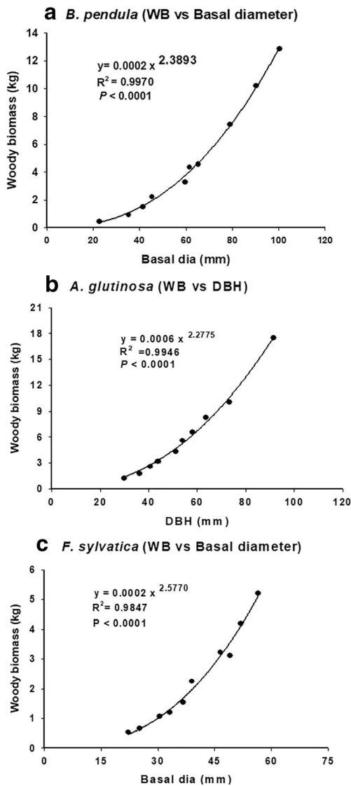
Fig. 5 Allometric relationship between plant variables and woody biomass (WB) of B. pendula , A. glutinosa and F. sylvatica . Scattered plots show data from ten selected plants and the best fitted lines with basal diameter for B. pendula and F. sylvatica and diameter at breast height (DBH) for A. glutinosa . The regression equations, coefficient of determination and P values (using ANOVA) are inserted in each panel
