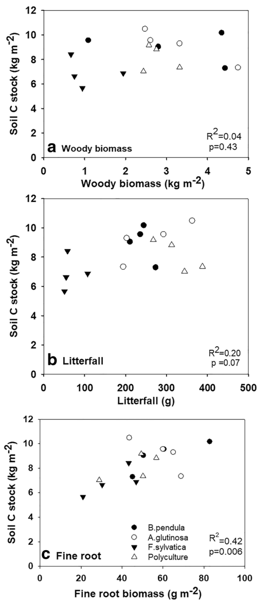
Fig. 4 Relationships between soil C stocks and: a aboveground woody biomass, b annual litter fall and c fine root (< 2 mm) biomass. Soil organic C stocks were measured in 16 mono- and polyculture stands in 0–50 cm depth
