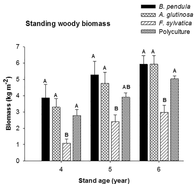
Fig. 2 Aboveground woody biomass in mono- and polyculture stands of B. pendula , A. glutinosa and F. sylvatica at the end of the 4th, 5th and 6th growing seasons. Woody biomass was estimated using species-specific allometric equations, developed by the tree harvesting approach after 6 years of stand age. Bars mean SE ( n = 4 ). Within 1 year, bars without the same indices are significantly different ( P < 0.05 )
