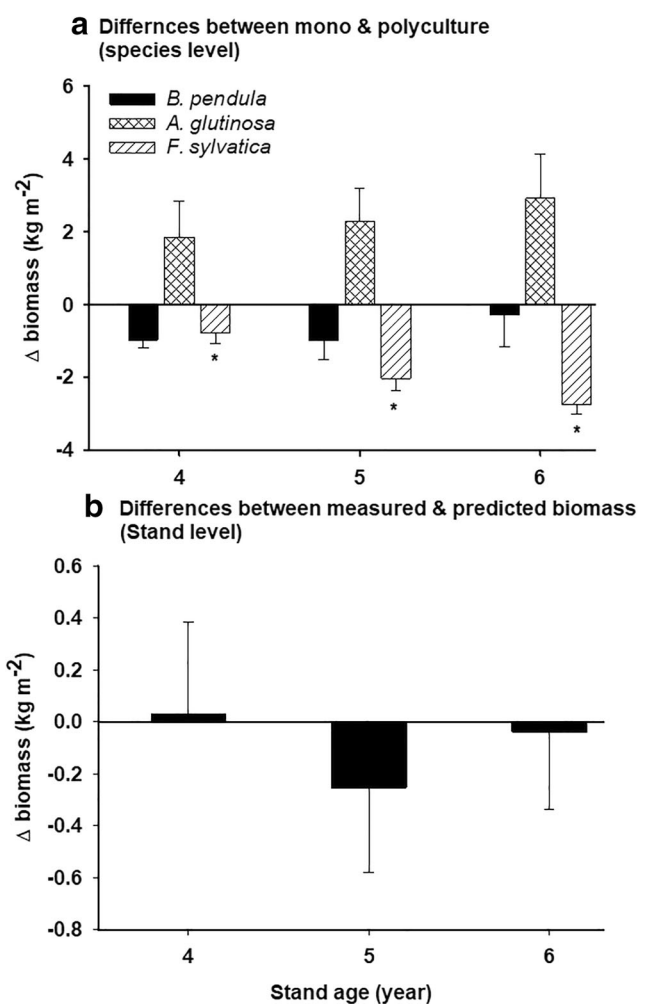
Fig. 3 Mixture effects in three-species polyculture (positive and negative values indicate higher and lower biomass in polyculture than monoculture respectively). a Species-level differences in biomass. F. sylvatica showed significant mixture effect (–ve differences) but A. glutinosa and B. pendula had insignificant impacts on biomass. b Stand-level mixture effect. The differences between measured (in polyculture stand) and predicted (calculated from monoculture stands) woody biomass, which were not statistically significant. Bars mean SE ( n = 4 ), Asterisk indicates statistically significant differences
