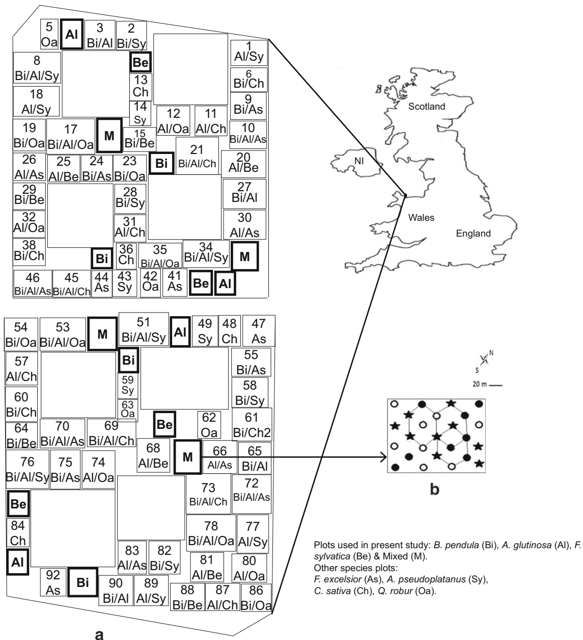
Fig. 1 Experiment site and plantation design. a Twelve monoculture of B. pendula (Bi), A. glutinosa (Al) and F. sylvatica (Be) and four three-species polyculture (M) plots, distributed over two plantation blocks. b
