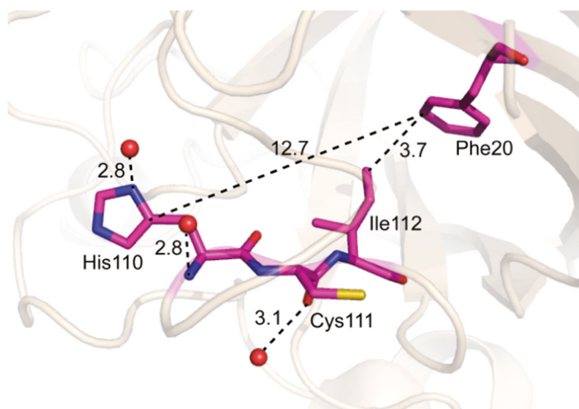
Figure 4. The modifications of residues, Phe20 and Ile112, with limited solvent accessibility (PDB: 1HL4). The numbers are the measured distances(Å). The graphic was generated using PyMOL software
