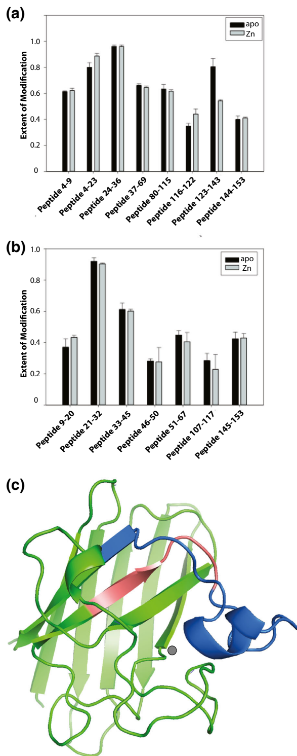
Figure 1. The electrostatic loop becomes less solvent accessible upon zinc binding. The figure shows the extent of modification of peptides from hSOD1 proteins irradiated in the presence of 5 mM H_2O_2 . The proteins were digested by trypsin (a) and chymotrypsin (b). The extent of modification was determined by comparing the intensities of unmodified peptides between irradiated and control samples (see Experimental Section, Figure S2) (c). The trypsin difference data was superimposed upon the hSOD1 monomer structure with blue representing the region less solvent accessible in the Zn-bound form (residues 123–143) while a short region that became more accessible is shaded in red (116–122). The graphic was generated from PDB 1HL4 using PyMOL software and shows a ribbon diagram of the monomer polypeptide backbone with Zn bound (gray disc). The structure 1HL4 was obtained by X-ray crystallography of the Zn-bound apo-hSOD1 [35]
