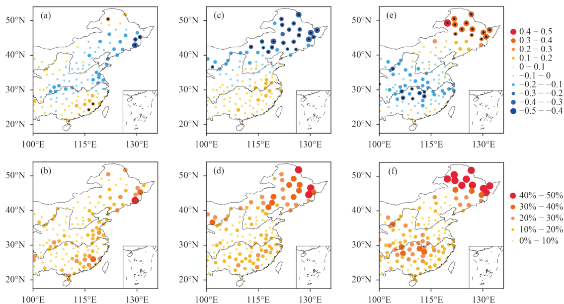
Fig. 6. As in Fig. 5, but for the summer SAT (°C).
