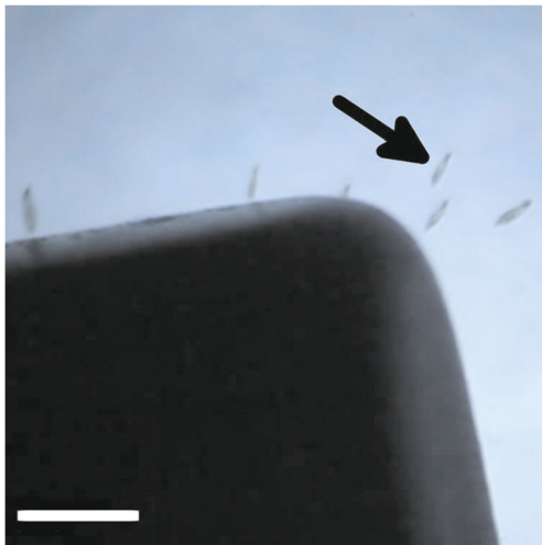
Fig. 3 Stereomicrograph showing MNP-treated P. caudatum cells (arrowed) being attracted towards a permanent magnet (black object). Scale bar 500 \mu\text{m}
