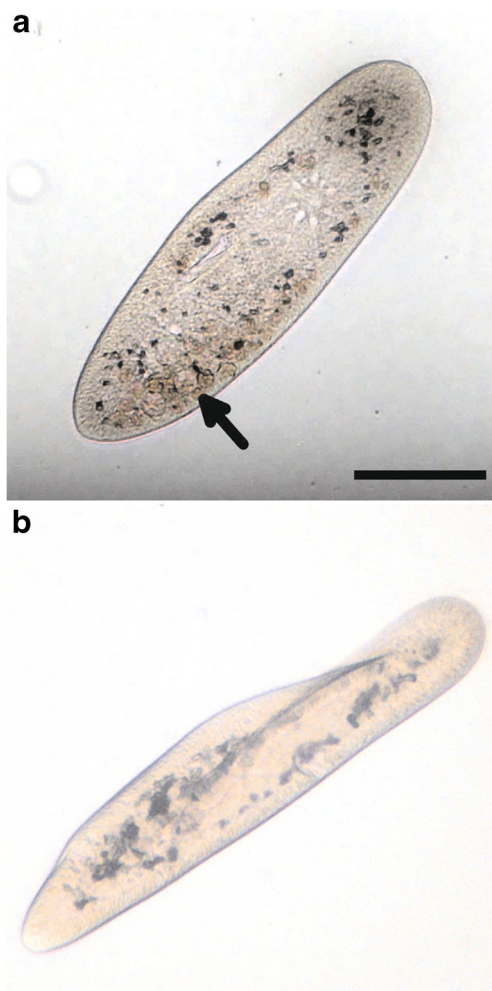
Fig. 1 Photomicrographs to show appearance of P. caudatum cells (unfixed): (a) Following exposure to MNPs. Multiple rust-coloured deposits (arrowed) are visible in the cytoplasm. (b) Control, demonstrating a lack of rust-coloured deposits. Scale bar 100 \mu\text{m}
