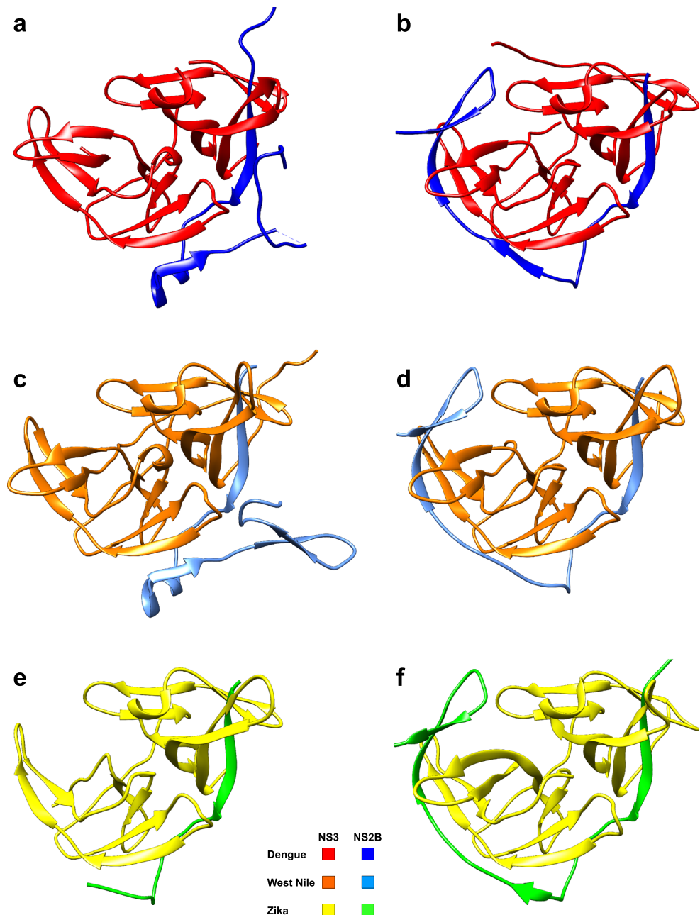
Fig. 2 X-ray crystal structures of inactive (open) and active (closed) conformations of flavivirus NS2B-NS3 proteases. Co-crystallised ligands have been removed from the active (closed) structures. (a) Inactive (open) conformation of the dengue protease serotype 2 (2FOM) (Erbel et al. 2006). (b) Active (closed) conformation of the dengue protease serotype 3 (3U11) (Noble et al. 2012). (c) Inactive (open) conformation of the West Nile protease mutant H51A (2GGV) (Aleshin et al. 2007). (d) Active (closed) conformation of the West Nile protease (5IDK) (Nitsche et al. 2017). (e) Inactive (open) conformation of the Zika protease (5GXJ) (Chen et al. 2016). (f) Active (closed) conformation of the Zika protease (5LC0) (Lei et al. 2016). This figure has been generated with Chimera (Pettersen et al. 2004)
