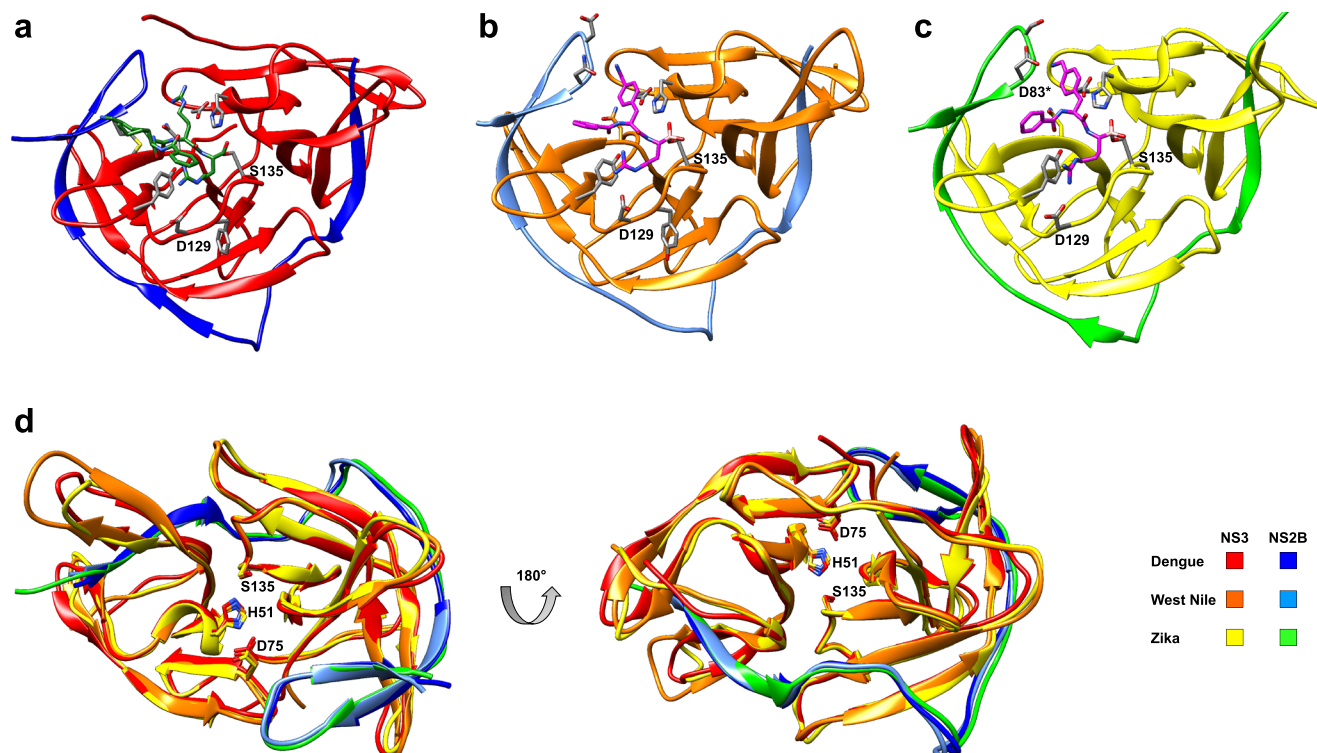
Fig. 1 Ligand-bound X-ray co-crystal structures of active flavivirus NS2B-NS3 proteases. (a) Dengue protease serotype 3 with the covalently bound aldehyde ligand 1 (3U1I) (Noble et al. 2012). (b) West Nile protease with the covalently bound boronate ligand 2 (5IDK) (Nitsche et al. 2017). (c) Zika protease with the covalently bound boronate ligand 2 (5LC0) (Lei et al. 2016). (d) Superimposition of active conformations
