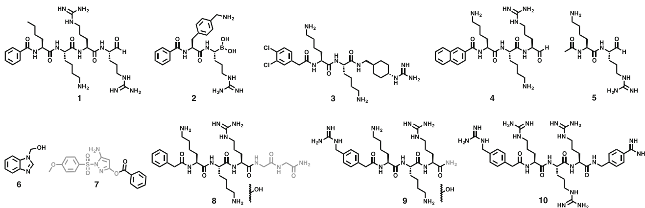
Fig. 4 Active-site inhibitors that were co-crystallised with NS2B-NS3 proteases from dengue, West Nile and Zika viruses. The actual observed ligand is highlighted in black. Inhibitor moieties that have been cleaved or
