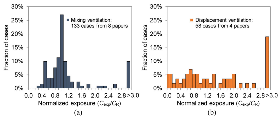
Fig. 1 The distribution of normalized personal exposure to exhaled contaminants for the 191 cases collected from the literature: (a) mixing ventilation and (b) displacement ventilation
