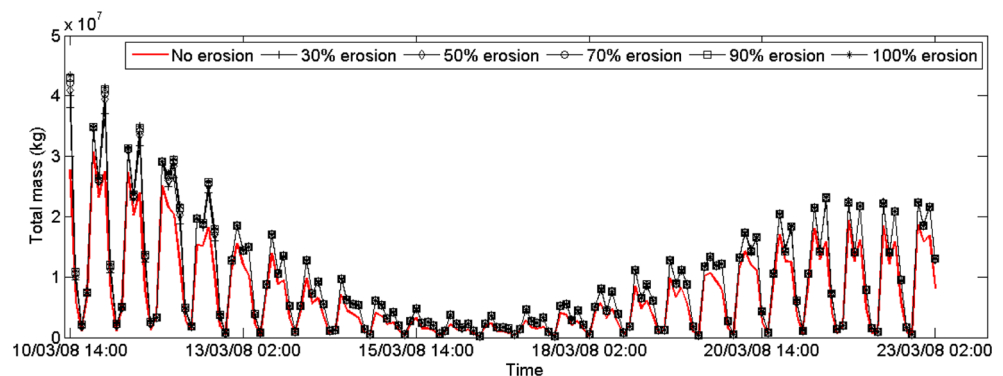
Fig. 6 Total mass of suspended sediment in the domain enclosing the salt marsh. Results are presented for six salt marsh erosion scenarios: no marsh erosion, 30% marsh erosion, 50% marsh erosion, 70% marsh erosion, 90% marsh erosion and 100% marsh erosion
