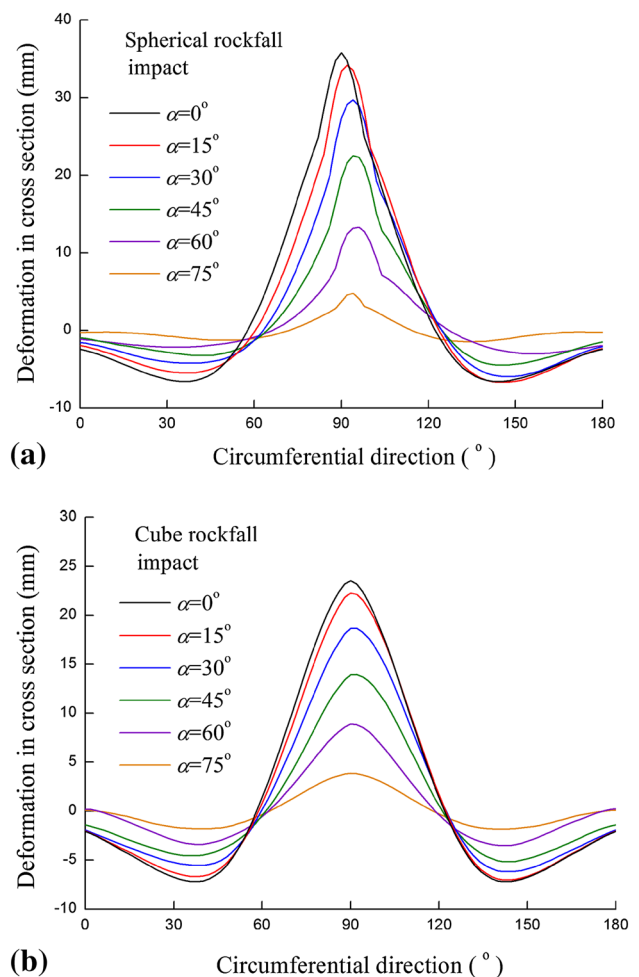
Fig. 15 Pipeline deformation in cross surface
