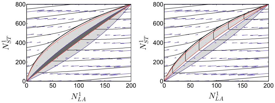
Fig. 7 Equilibrium region (dark gray) in Venue 1 with \xi_1 = -3.5 and Venue 2 (not shown) without Last Look, and c = 0.05 and 0.025 in the left and right panels. The other parameters are \sigma = 1 , \beta = 0.8 , \rho = 0.5 , \kappa_{LA} = 40 , \kappa_{ST} = 20 , and \delta = 0.5 |\xi| . Black lines indicate the migration of traders. Blue arrows indicate the direction of the migration. Red lines bound the equilibrium region for LAs, blue lines bound the equilibrium region for STs. (Color figure online)
