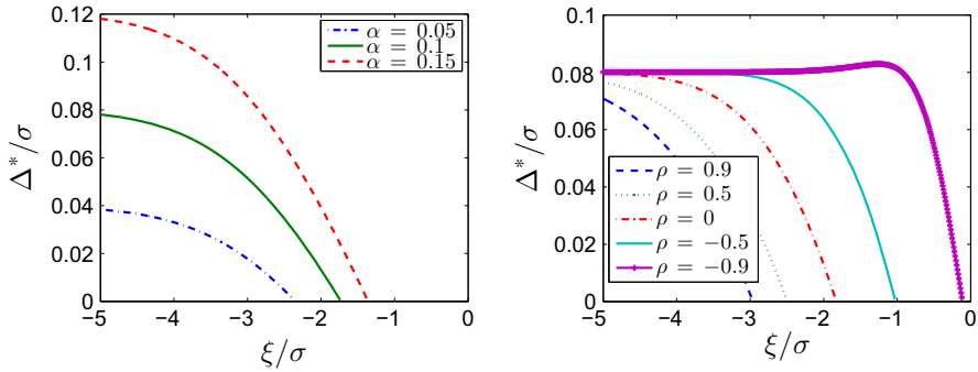
Fig. 3 Optimal spread \Delta^* (relative to \sigma ) which renders the broker’s expected loss to LAs equal to her expected gains from STs. Recall that \alpha is the percentage of LAs in the market. Here, \beta = 0.8 , in the left panel \rho = 0.5 , and in the right panel \alpha = 0.1
