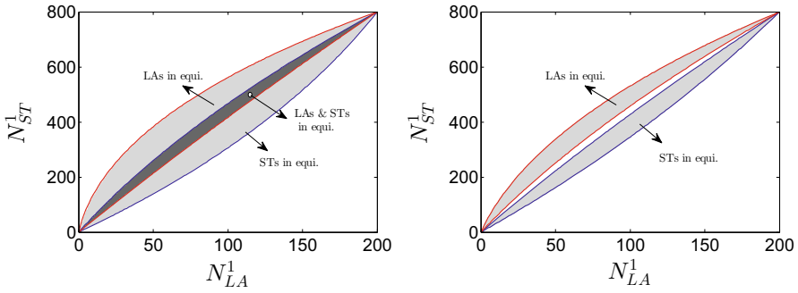
Fig. 6 Equilibrium region (dark gray) in Venue 1 with \xi_1 = -3.5 and Venue 2 (not shown) has no Last Look. Left panel migration cost is c = 0.05 , and right panel c = 0.025 . The other parameters are \sigma = 1 , \beta = 0.8 , \rho = 0.5 , and \delta = 0.5 |\xi| . Red lines bound the equilibrium region for LAs, blue lines bound the equilibrium region for STs. (Color figure online)
