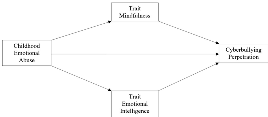
Fig. 1 Hypothesized model
