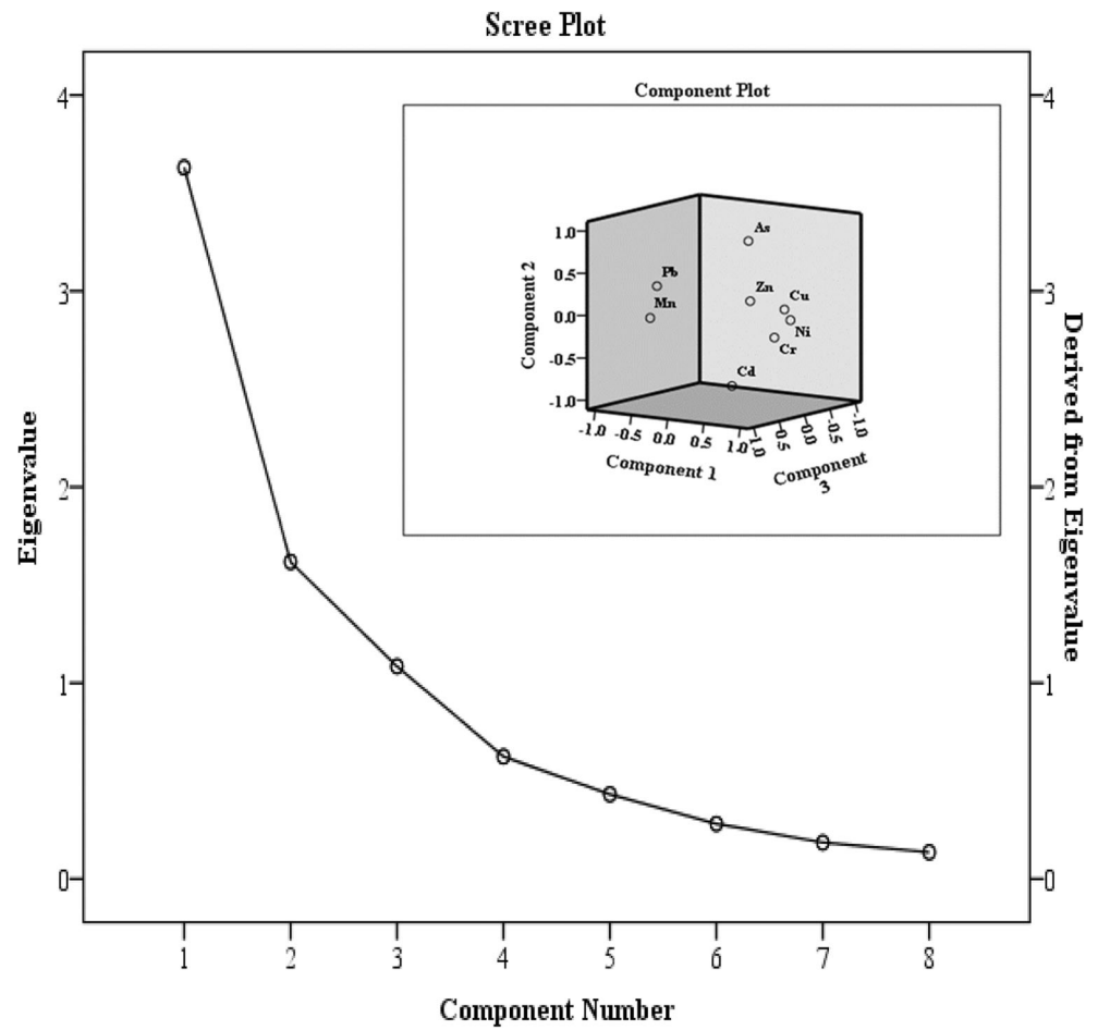
Fig. 4 Scree plot of heavy metals in sediments. The graph shown in upper right corner shows the concentration of principle components variables in a loading plot
