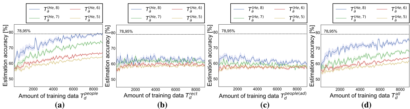
Fig. 18 Prediction accuracy for each T_a^S ( S = 5, 6, 7, 8 ) with (a) T_d^{people} , (b) T_d^{rect} , (c) T_d^{people(ad)} , and (d) T_d^{all}
