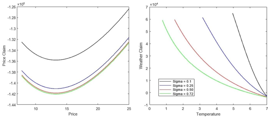
Fig. 4 Tails of price and weather contingent claims for different values of volatility sigma. Left: Price claim, right: Weather claim
