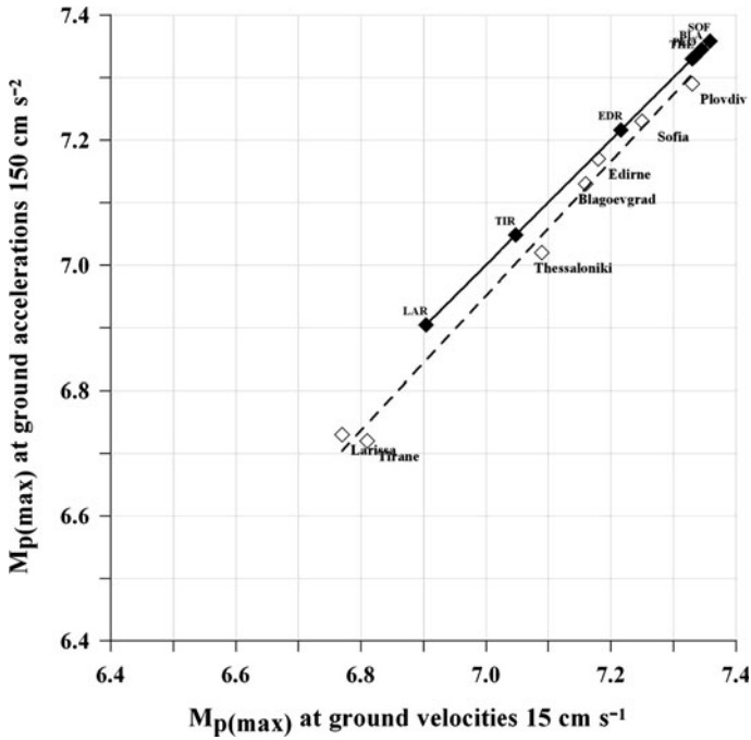
Fig. 21 Linear correlation of a minimum and b maximum most perceptible earthquake magnitude for horizontal ground acceleration and horizontal ground velocity for a nominal earthquake of 15-km focal depth. The solid line is the best-fit through maximum credible magnitude data points ( M_3 ) derived from the summation of cumulative seismic moment release in the considered area; dashed line is the best-fit through most perceptible earthquake magnitude ( M_{P(\max)} ) data points
