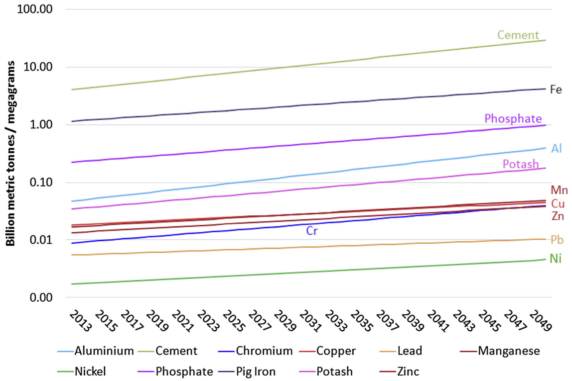
Figure 2. World production scenario 2013–2050, expressed in billion metric tonnes per megagram of a selection of minerals and metals required for infrastructure, building, mass-produced industrial goods or agriculture. Y scale is logarithmic. Compiled from USGS data.
