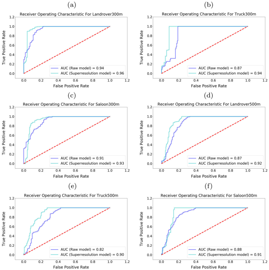
Fig. 11 ROCs for the 300 m (a, b, c) and 500 m (d, e, f) datasets of Truck, Saloon and Landrover in Trial 2. Each graph features two ROCs corresponding to raw model and super-resolution model-derived results
