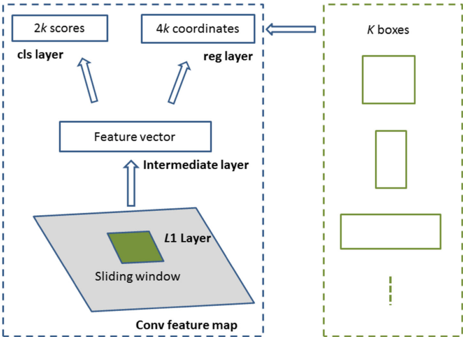
Fig. 8 Region Proposal Network (RPN)
