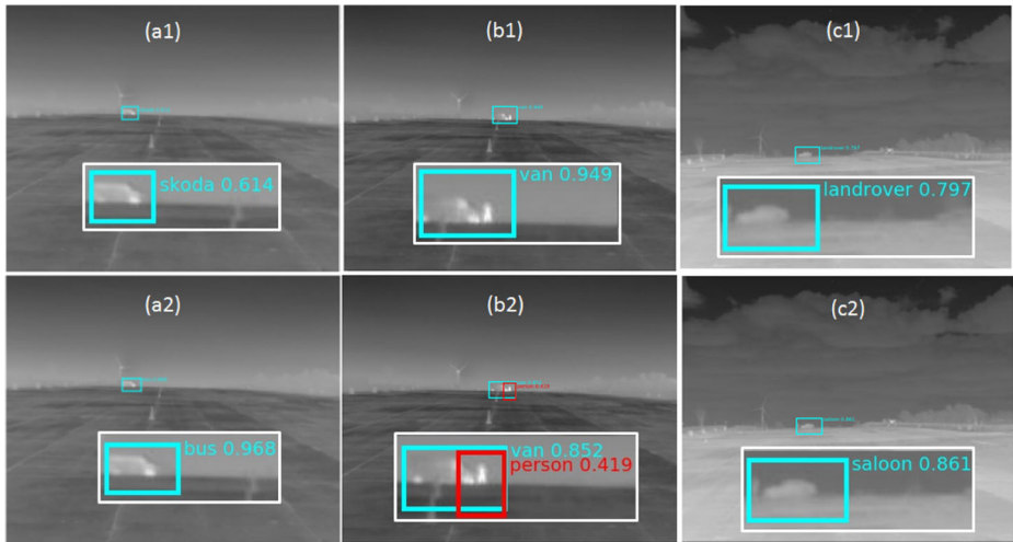
Fig. 15 Examples showing the performance of the superresolution-model. Upper row: the results for Skoda600m, Van600m, Saloon600 m with the raw-model. Lower row: the results for the same images with the superresolution-model
