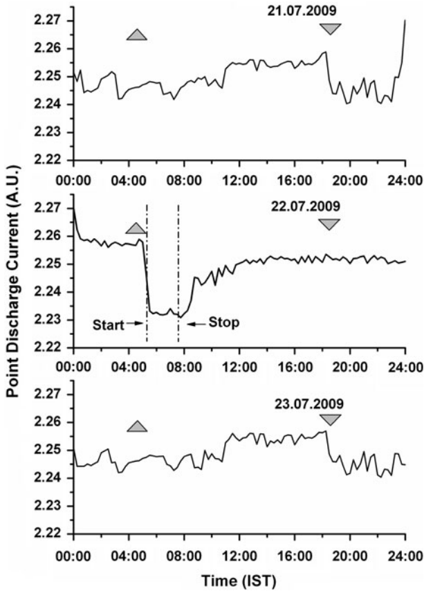
Fig. 4 Temporal variation of point discharge current over Kolkata is presented by the continuous line curve during solar eclipse on July 22, 2009 ( middle panel ). The upper and the lower panel are for the two control days, July 21 and 23, 2009, respectively. Upper and lower triangle marks are for local sunrise and sunset
