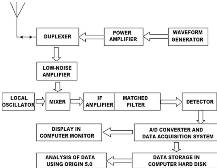
Fig. 1 Block diagram of the receiving system
