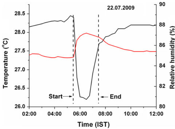
Fig. 3 Temporal variation of temperature ( black coloured curve ) and relative humidity ( red coloured curve ) on July 22, 2009, the day of eclipse between the period of 02:00 IST and 12:00 IST. (Color figure online)
